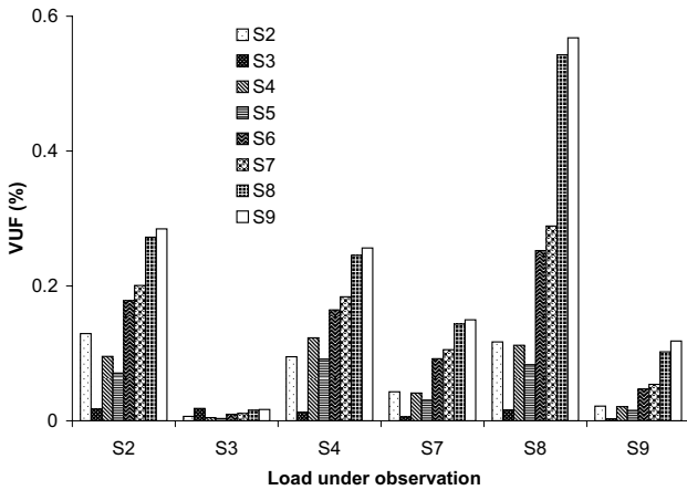
Fig. 7. Nodal voltage unbalance levels caused by the individual loads
