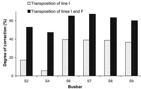
Fig. 14. Nodal degree of correction arising due to proposed mitigation options
