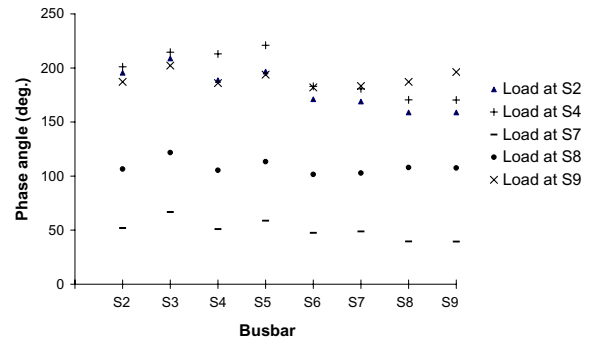
Fig. 8. Phase angles of nodal negative sequence voltages caused by the individual loads
