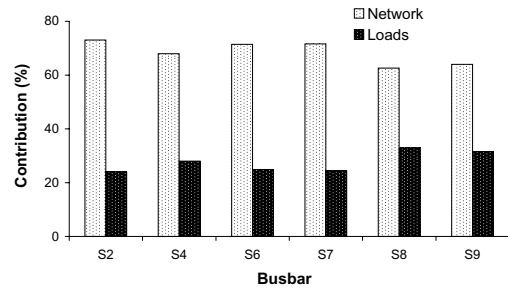
Fig. 11. Nodal contribution made individually by the network and the loads to the resultant voltage unbalance levels
