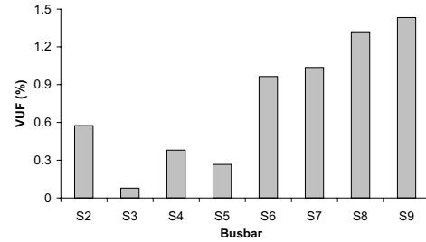
Fig. 2. Nodal voltage unbalance levels arising as a result of the asymmetrical network
