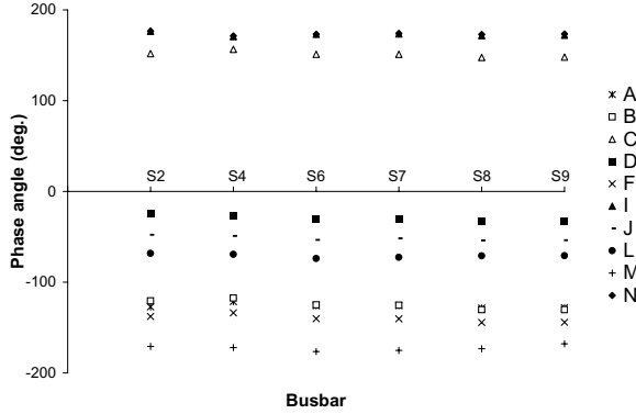
Fig. 4. Phase angles of nodal negative sequence voltages caused by the individual lines
