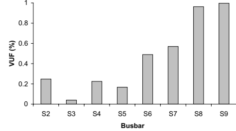
Fig. 6. Nodal voltage unbalance levels arising as a result of the unbalanced loads alone
