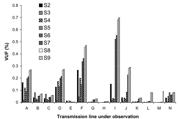
Fig. 3. Nodal voltage unbalance levels caused by the individual transmission lines
