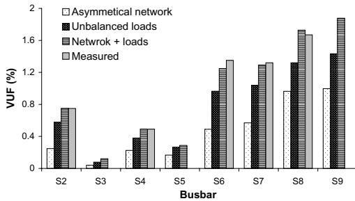
Fig. 10. Nodal voltage unbalance levels arising as a result of the interaction of the asymmetrical network and the unbalanced loads in comparison to that caused alone by the asymmetrical network and the unbalanced loads, and also to the measured values
