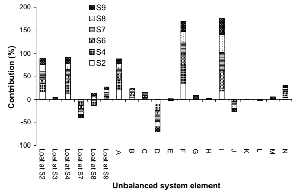
Fig. 12. Nodal contribution of individual unbalanced elements (lines and loads) to the resultant voltage unbalance levels
