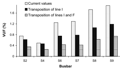
Fig. 13. Nodal residual voltage unbalance levels arising due to proposed mitigation options, in comparison to the current voltage unbalance levels
