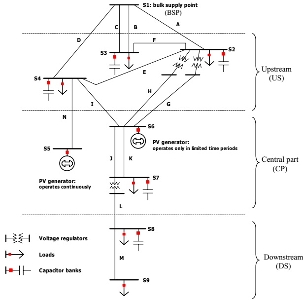
Fig. 1. 66kV sub-transmission system under study
