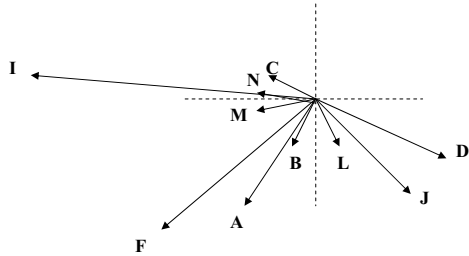
Fig. 5. Representation of overall voltage unbalance behaviour of the individual lines
