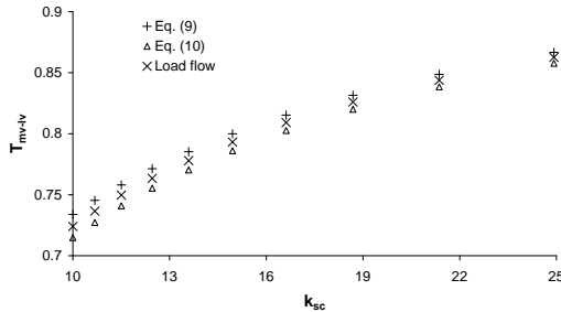
Fig. 4. Variation of T_{mv-lv} with k_{sc} in relation to a load base with Z-10%, I-5%, PQ-15% and IM-70%
