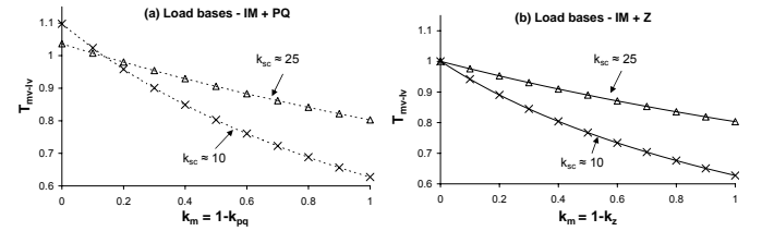
Fig. 6. Variation of T_{mv-lv} (a) with k_m = 1 - k_{pq} (b) with k_m = 1 - k_z , for two cases where k_{sc} \approx 25 and k_{sc} \approx 10
