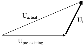
Fig. 1. Emission level, as defined in IEC/TR 61000-3-13, from an unbalanced installation
