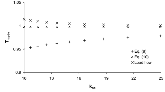
Fig. 5. Variation of T_{mv-lv} with k_{sc} in relation to a load base with Z-25%, I-5%, PQ-60% and IM-10%
