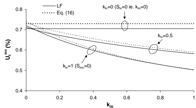
Fig. 9. Variation of U_t^{mv} with k_m for k_{lv} = 1 , k_{lv} = 0.5 and k_{lv} = 0
