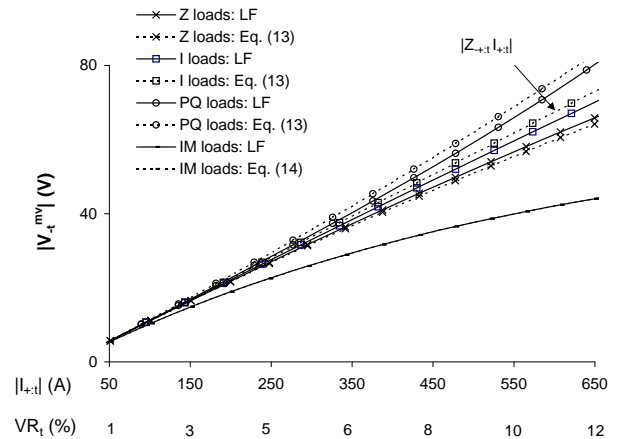
Fig. 8. Variation of |V_{-t}^{mv}| with |I_{+:t}| ( VR_t values corresponding to various |I_{+:t}| are also indicated) in relation to the four basic load types
