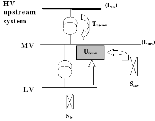
Fig. 2. Simple illustration of determination of allowed global contribution [5]
