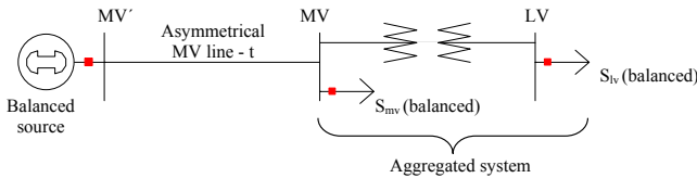
Fig. 7. MV-LV radial power system
