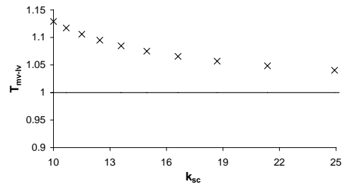
Fig. 3. Variation of T_{mv-lv} with k_{sc} in relation to a load base containing constant power elements with 0.9 lag. pf
