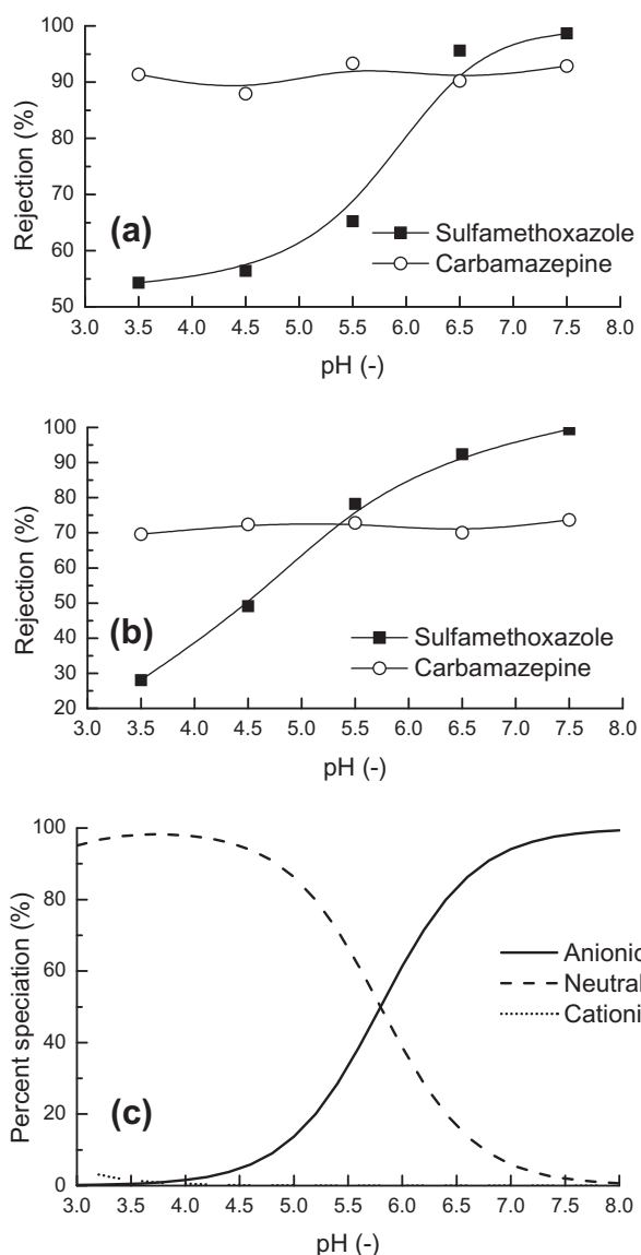
Fig. 6. Rejection sulfamethoxazole and carbamazepine in (a) FO mode, (b) PRO mode as a function of feed pH and (c) the speciation of sulfamethoxazole as a function of pH. The data points represented the rejection at the end of 10-h experiments (experimental conditions were as per Fig. 4).
