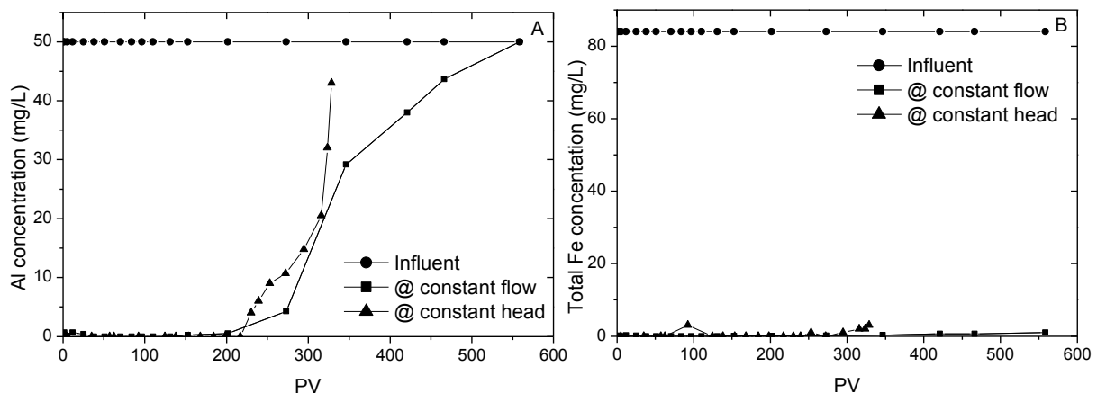
Figure 3. (A) Al and (B) Total Fe concentrations vs. number of pore volume
