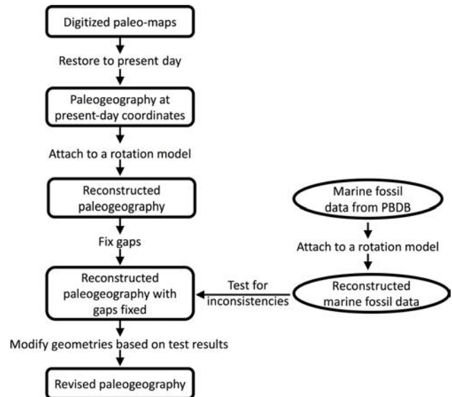
Figure 2. Workflow used to transfer a set of paleogeographic geometries from one reconstruction to another, followed by revision using paleoenvironmental information indicated by marine fossil collections from the Paleobiology Database (PBDB).
