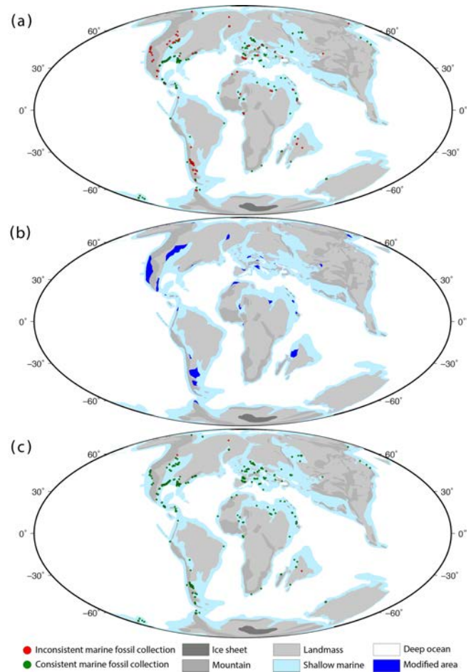
Figure 4. (a) Test between the global paleogeography at 76 Ma reconstructed using the plate motion model of Matthews et al. (2016) with gaps fixed and the paleoenvironments indicated by the marine fossil collections from the PBDB. (b) Area modified (blue) to resolve the test inconsistencies. (c) Test between the revised paleogeography at 76 Ma and the same marine fossil collections. Mollweide projection with 0^\circ E central meridian.
