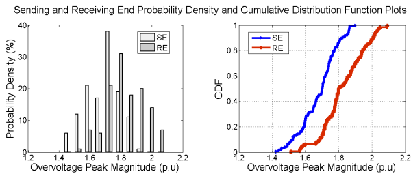
Fig. 5. PD/CDF of overvoltage peaks (8th aiming point of 0.8 ms pole span)
