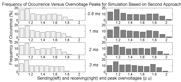
Fig. 4. Frequency of occurrence of overvoltage peaks from second approach.
