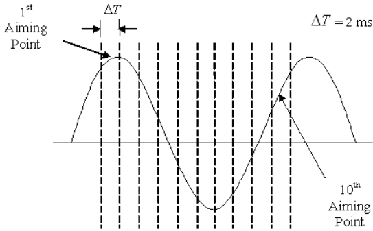
Fig. 1. Single phase view of aiming point settings for 2 ms pole span.
