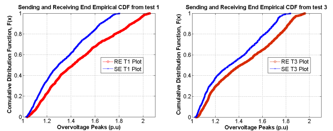
Fig. 3. CDF for Test 1 and Test 3 energisation schemes
