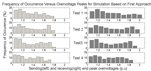
Fig. 2. Frequency of occurrence of overvoltage peaks from first approach.
