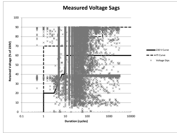
Figure 11: Measured Voltage Sags Plotted on Depth-Duration Plane
