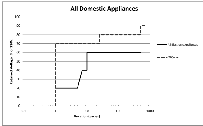
Figure 5: Voltage Sag Susceptibility Envelope for all Domestic Appliances
