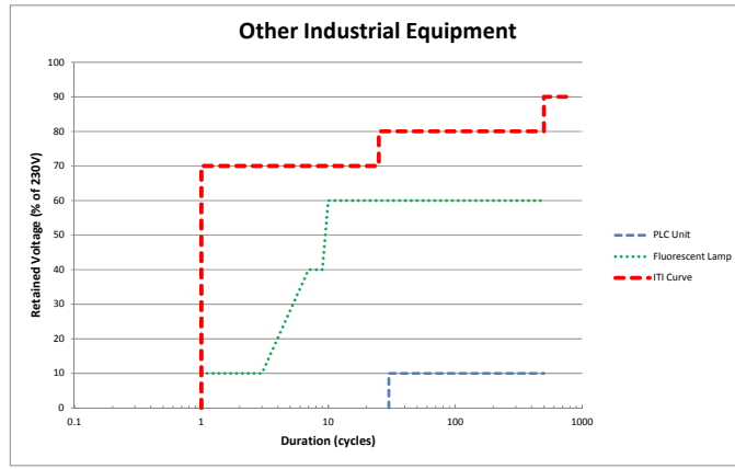
Figure 7: Voltage Sag Susceptibility Envelopes for Industrial Equipment (excluding contactors)
