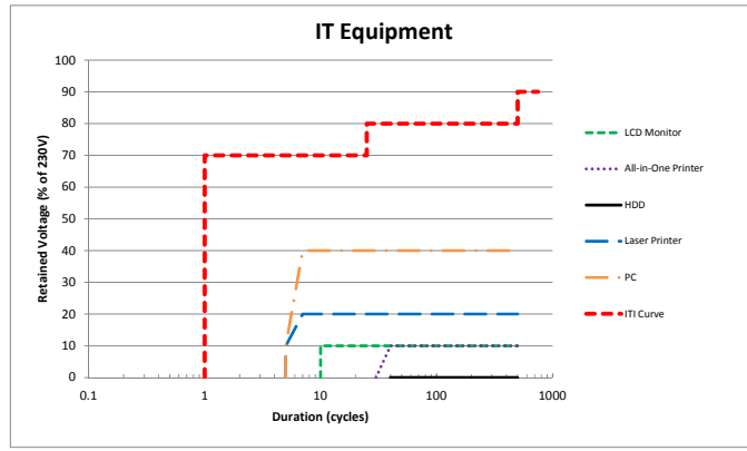
Figure 2: Voltage Sag Susceptibility Envelopes for IT Equipment
