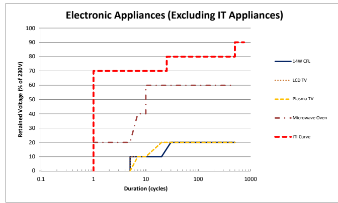
Figure 3: Voltage Sag Susceptibility Envelopes for Electronic Appliances (excluding IT appliances)
