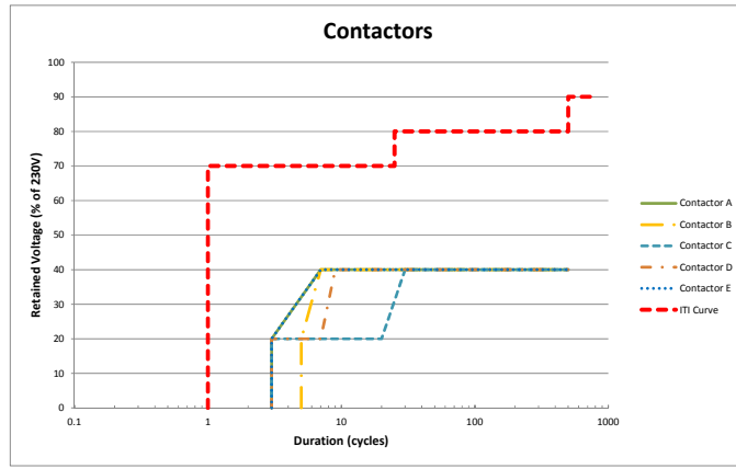
Figure 6: Voltage Sag Susceptibility Envelopes for Contactors
