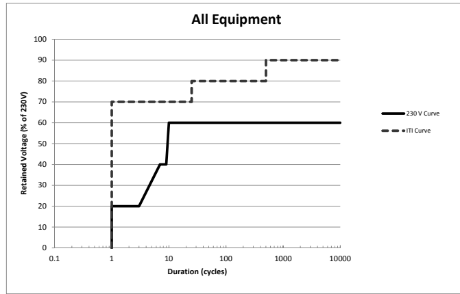
Figure 9: Voltage Sag Susceptibility Curve for all Tested Equipment (excluding VSDs)
