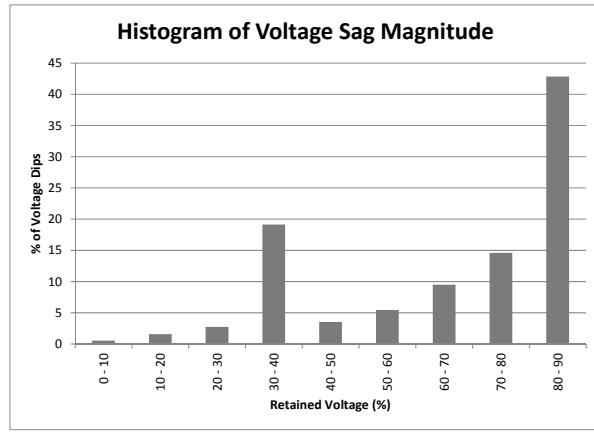
Figure 10: Histogram of Voltage Sag Magnitude
