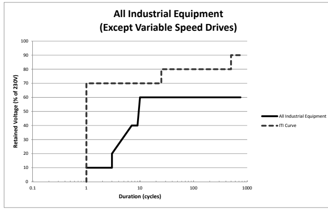
Figure 8: Voltage Sag Susceptibility for all Industrial Equipment (excluding variable speed drives)
