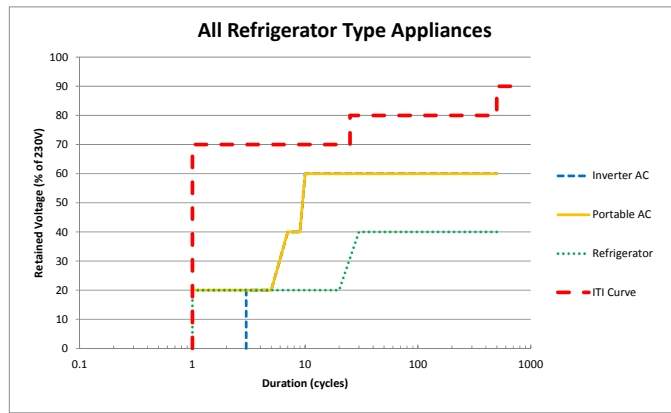
Figure 4: Voltage Sag Susceptibility Envelopes for Refrigerator Type Appliances
