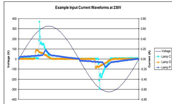
Figure 1: Selected CFL Input Current Waveforms
