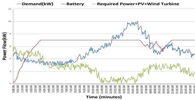
Fig. 9. Power flow after implementing predictive control algorithm.
