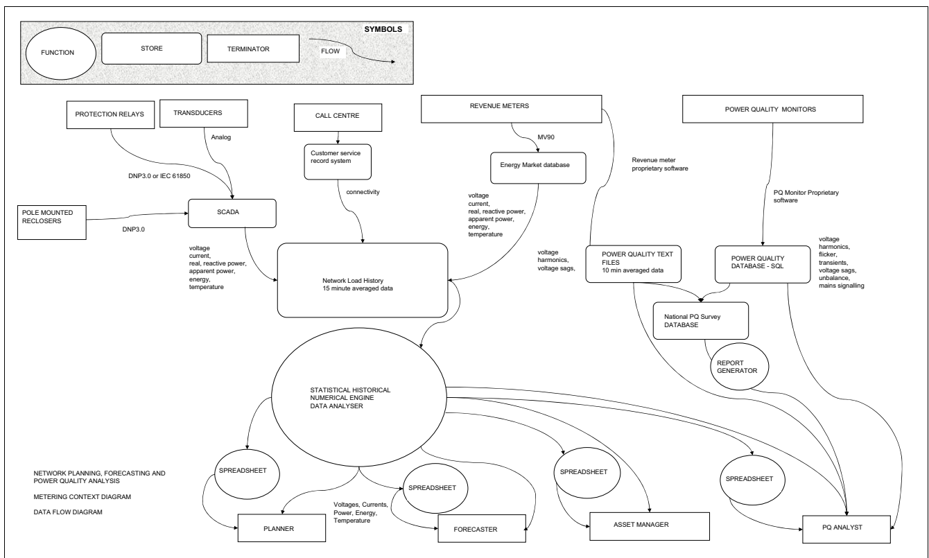
Fig. 4. Metering Data Flow Diagram of Future System
