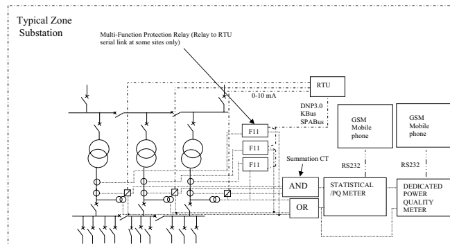
Fig. 2. Typical Zone Substation Monitoring
