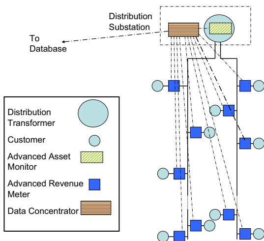
Fig. 1. Typical Low Voltage Distribution System Monitoring
