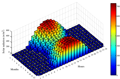
Fig. 7. Hourly average solar radiation
