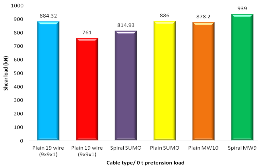
Figure 4: Peak shear loads of different types of cable bolts subjected to 0 t pretension load
