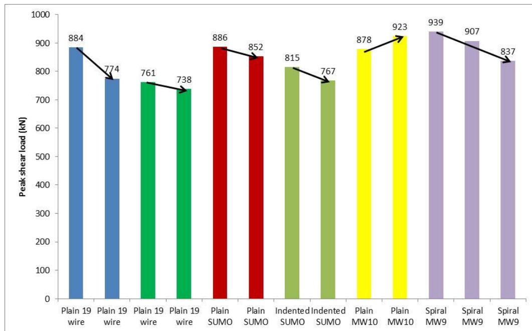
Figure 3: Effect of pretension load on peak shear load
