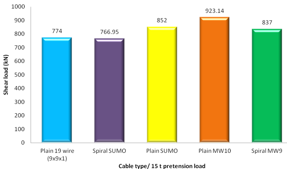
Figure 5: Peak shear loads of different types of cable bolts subjected to 15 t pretension load
