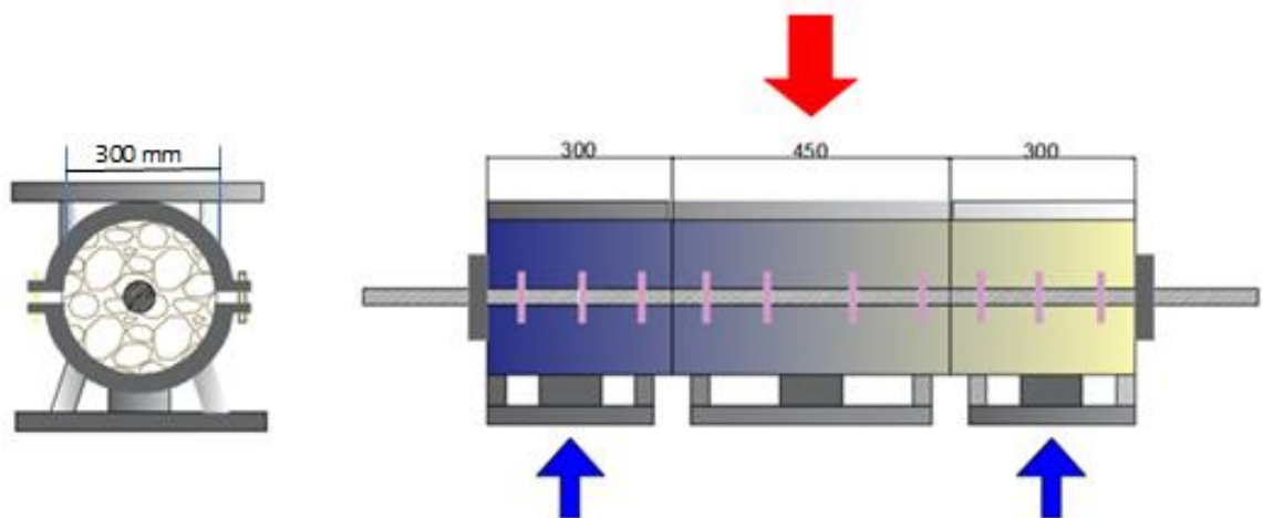
Figure 9: Double shear apparatus MKIV
