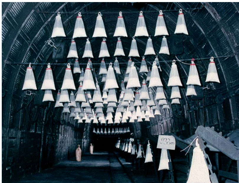
Figure 5: Bagged stone dust barrier (Belle and Du Plessis, 1999)
