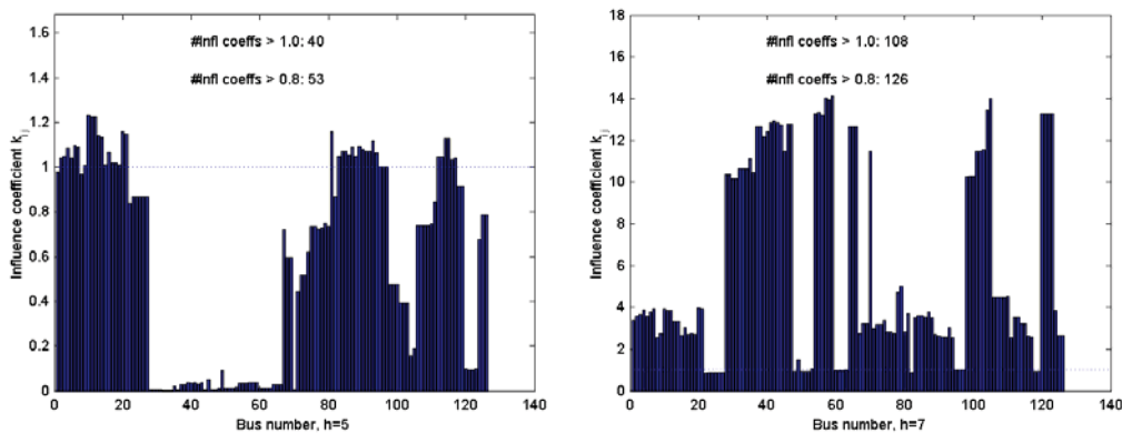
Figure 2: Influence coefficients calculated from a particular busbar to all busbars in study system at selected harmonics
