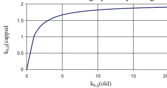
Figure 3: Relationship between uncapped and capped influence coefficients
