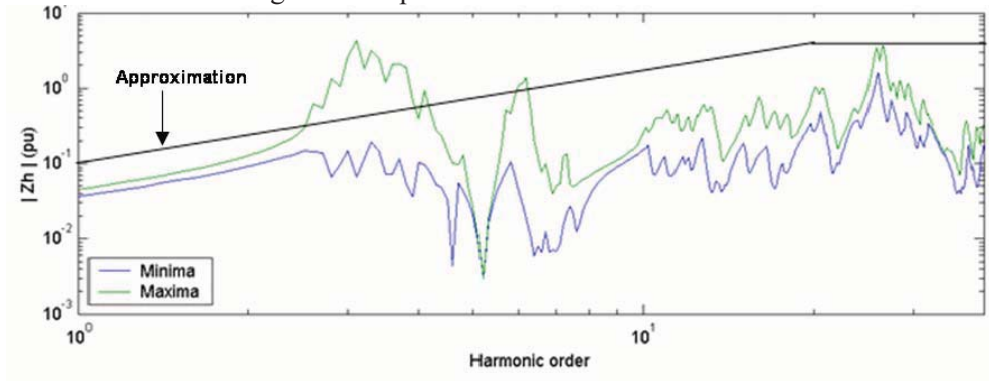
Figure 4: Harmonic impedance variation and approximation of (9)
