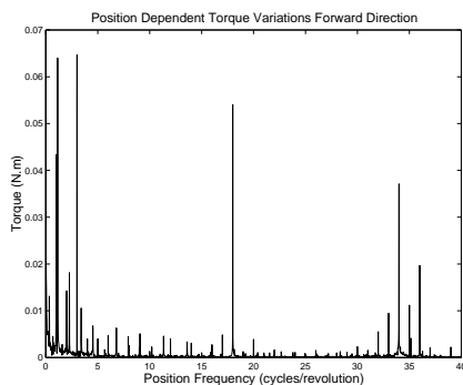
Figure 10: Ball screw Axis Frequency Spectrum
