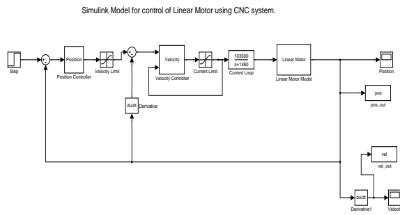
Figure 4: Simulink Model for Linear Motor System
