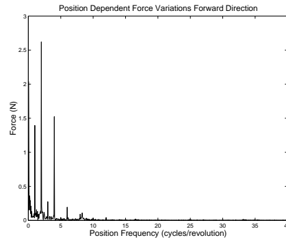
Figure 9: Linear Motor Frequency Spectrum
