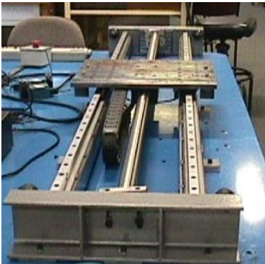
Figure 1: Linear Motor Test-Bed
