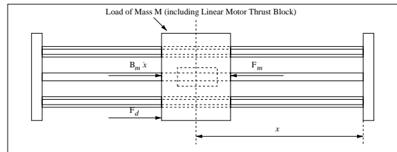
Figure 2: Diagram of Linear Motor Test-Bed
