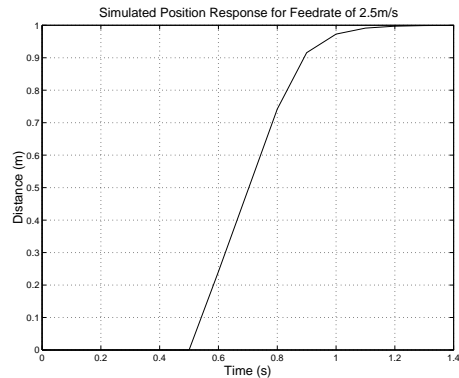
Figure 5: Simulated Position (Feed = 2.5m/s)
