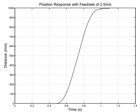
Figure 6: Experimental Position (Feed = 2.5m/s)
