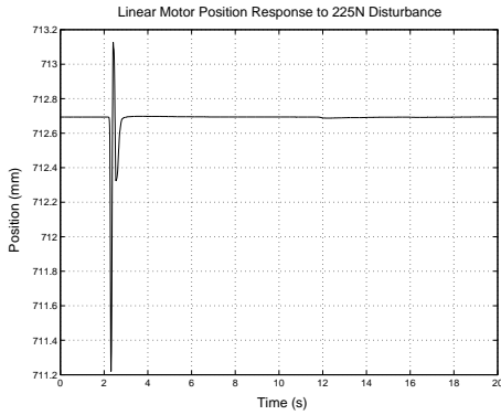
Figure 7: Linear Motor Position (225N Disturbance)
