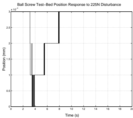
Figure 8: Ball Screw Axis Position (225N Disturbance)
