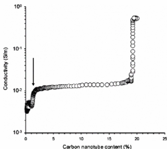
Fig. 1. Log of conductivity as a function a function of carbon nanotube content (% weight) for a gellan gum-CNT hydrogel. The arrow indicates the percolation threshold.
