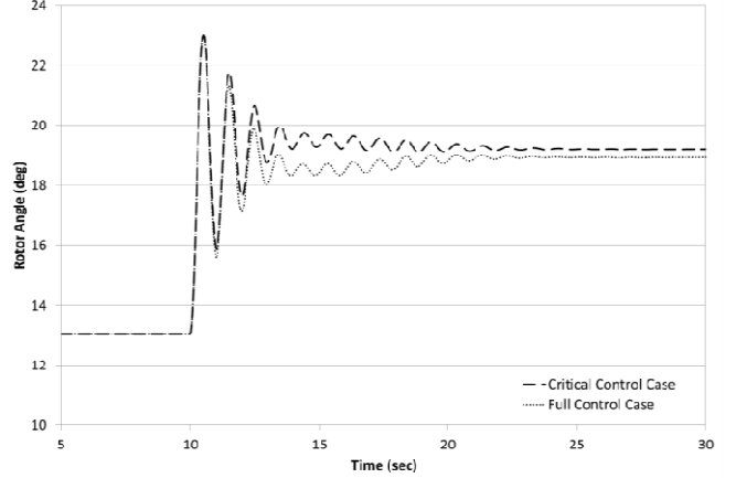
Fig. 3. Rotor angle traces for the generator at bus 34 following the loss of the generator at bus 32.
