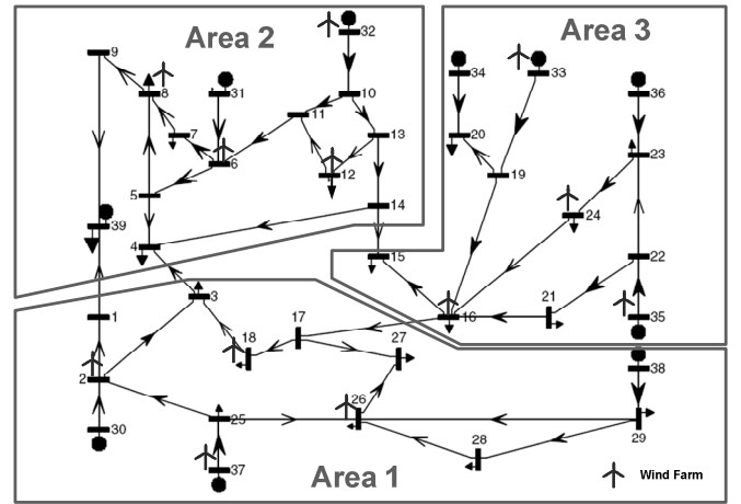
Fig. 1. New England 39 test system
