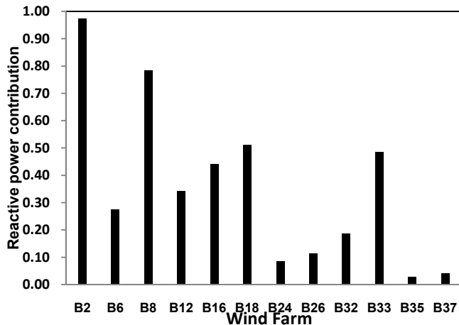
Fig. 5: Reactive power contribution of wind farms for optimization strategy 1
