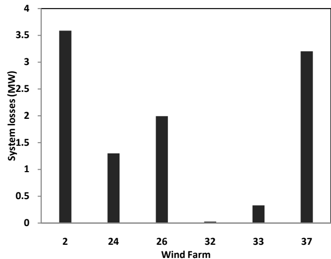
Fig. 9: System loss variation with voltage control at each wind farm location
