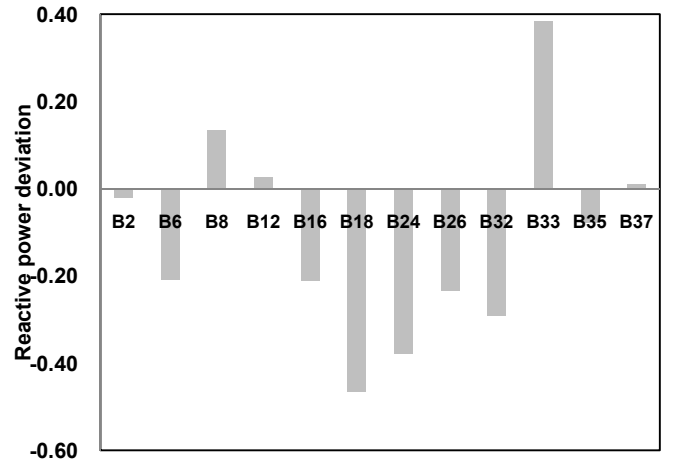
Fig. 7: Reactive power dispatch difference between two optimization strategies
