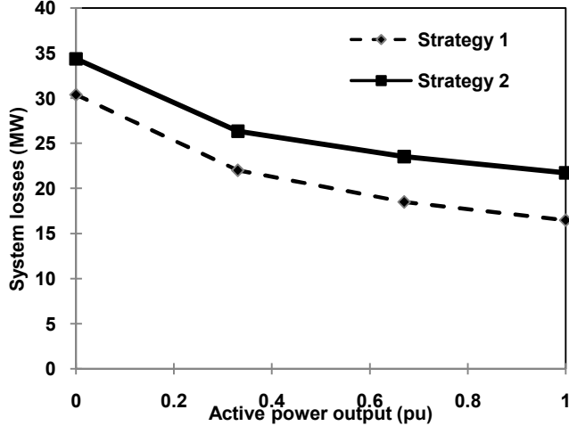
Fig. 4: Active power loss variation with wind farm power output
