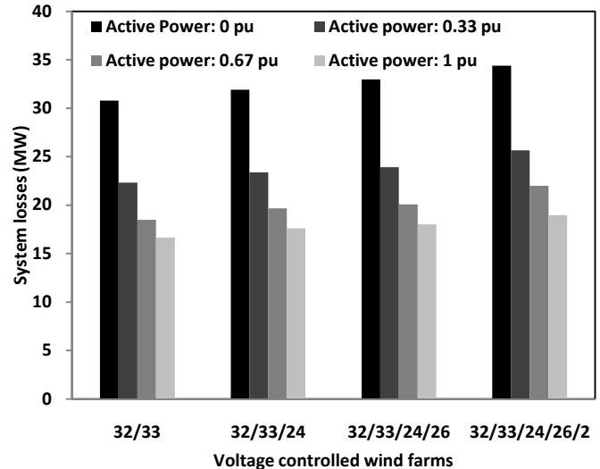
Fig. 10: System losses with selective voltage control
