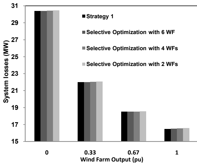
Fig. 8: System losses with selective optimization.
