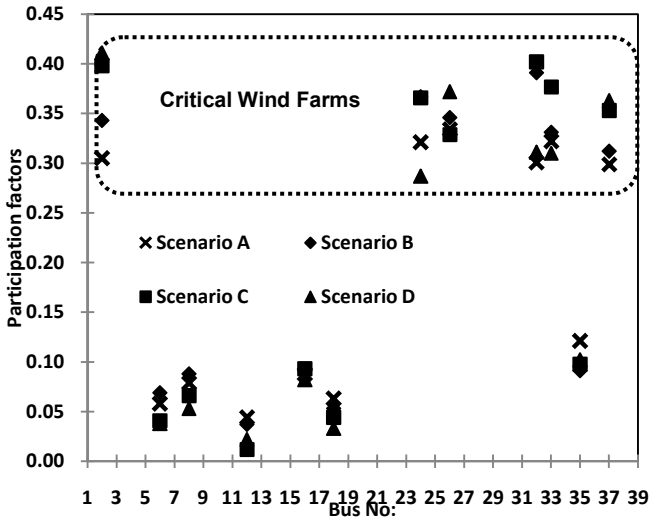
Fig. 2. Recorded participation factors for wind farms
