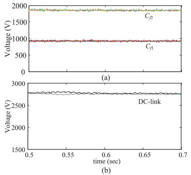
Fig. 6. Grid connected seven-level ANPC converter, (a) Flying capacitor voltages, (b) DC-link capacitor voltages
