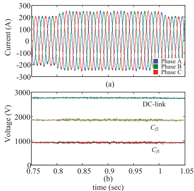
Fig. 11. Converter performance during a voltage sag at the PCC (a) Phase currents, (b) DC-link and flying capacitor voltages
