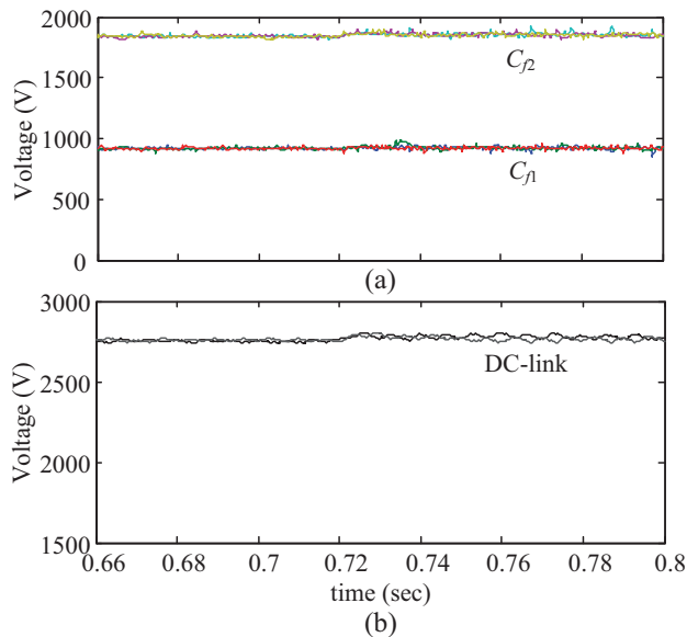
Fig. 9. Step change in the active power, (a) FC voltages, (b) DC-link capacitor voltages
