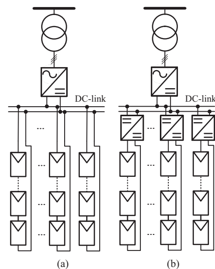
Fig. 1. PV system configuration (a) central inverter, (b) multistring inverter
