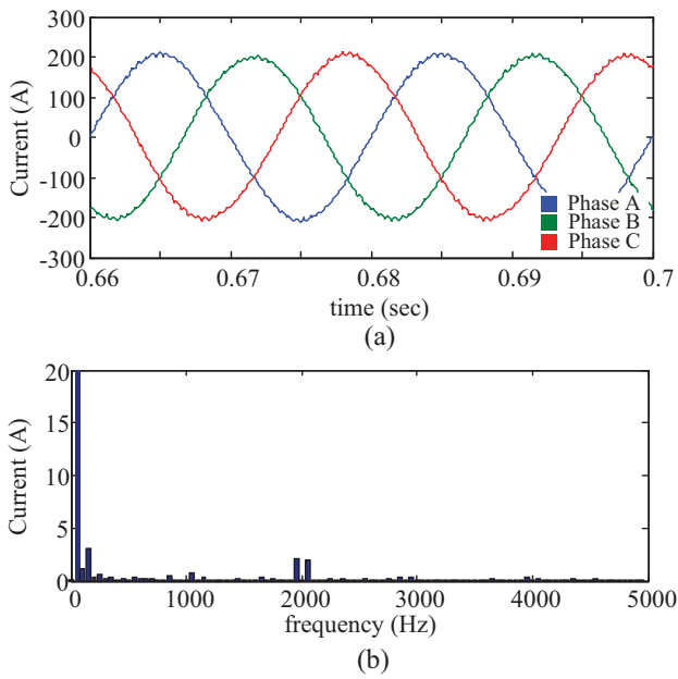
Fig. 4. Grid connected seven-level ANPC converter, (a) Grid currents, (b) Corresponding harmonic spectrum
