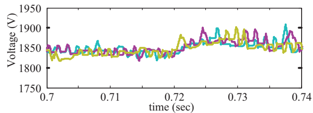
Fig. 10. Variation of cell two capacitor during a step change in active power
