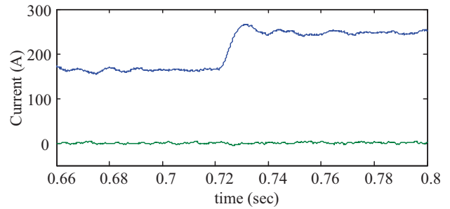
Fig. 7. d and q components of the grid currents for a step change in the active power of the converter
