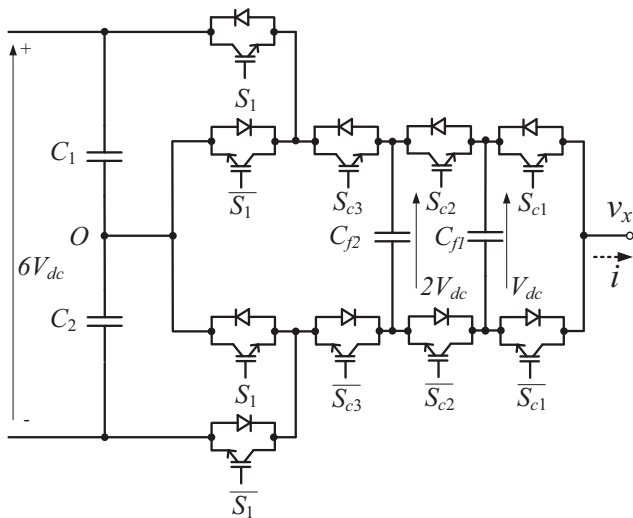
Fig. 2. Configuration of one phase of the seven-level flying capacitor based active NPC converter
