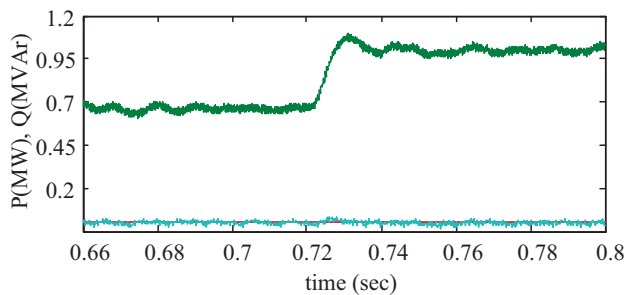
Fig. 8. Active and reactive power at the point of common coupling
