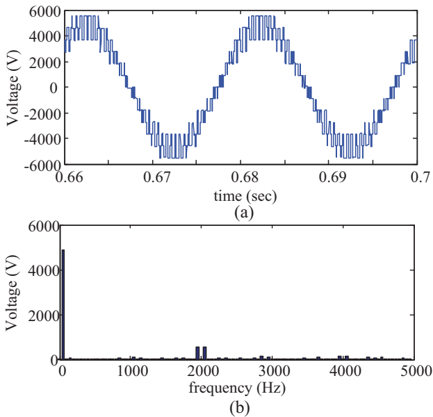
Fig. 5. Grid connected seven-level ANPC converter, (a) Line-to-line voltages, (b) Corresponding harmonic spectrum
