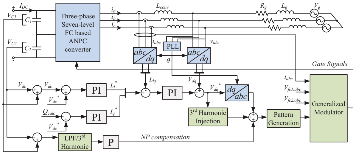
Fig. 3. Converter and controller configuration for the seven-level FC based ANPC converter
