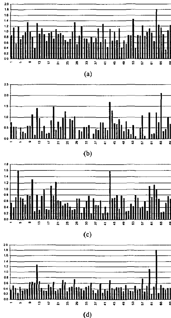
Fig. 2 Consolidated Indices for Individual Disturbances (a) Voltage V, (b) Unbalance U, (c) Flicker F, (d) Harmonics H (Horizontal axis gives site number, vertical scale gives normalized and consolidated index)
