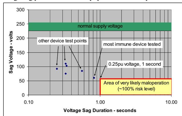
Fig. 8. Voltage Sag Immunity of a Range of Electronic Equipment
