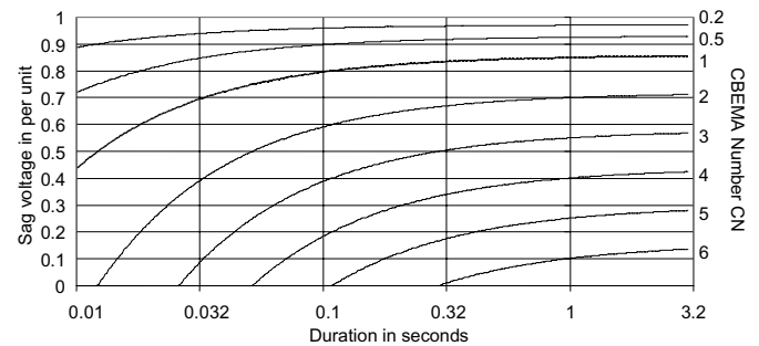
Fig. 6. CBEMA Number Contours
