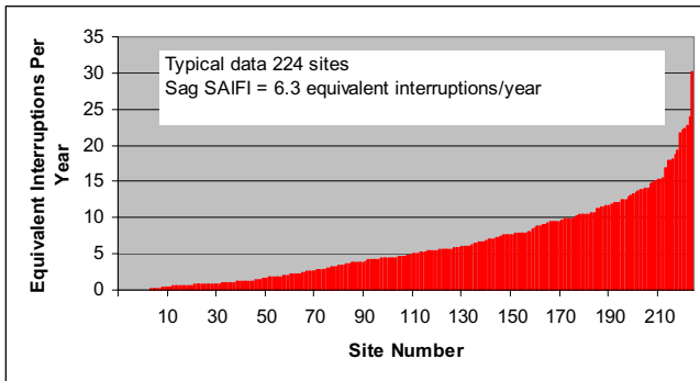
Fig. 10. Typical Sag SAIFI Distribution for a Large Number of Sites
