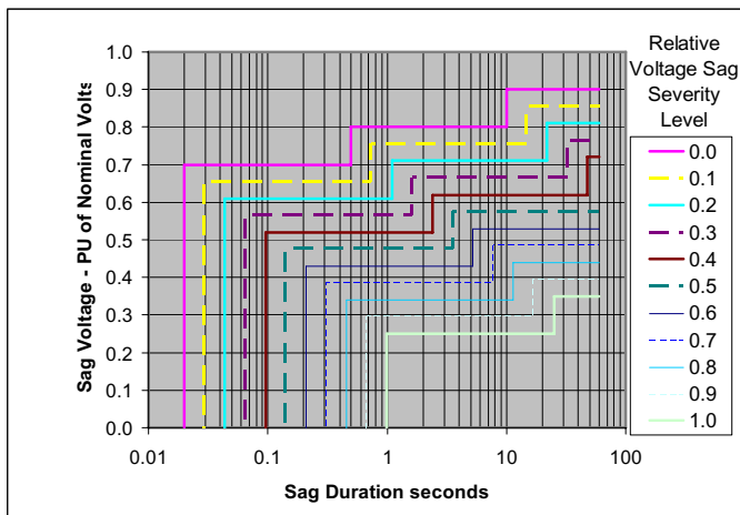
Fig. 9. Sag SAIFI Model – Voltage Sag Severity Levels
