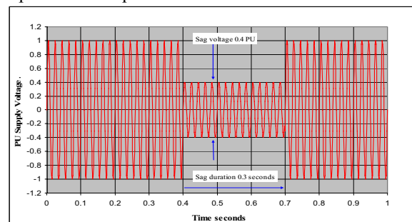
Fig. 1. Typical voltage sag waveform
