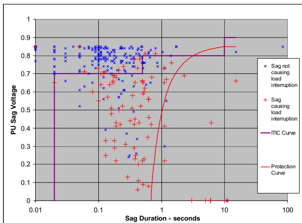
Fig. 7. ITIC Curve and voltage sags causing industrial plant interruptions
