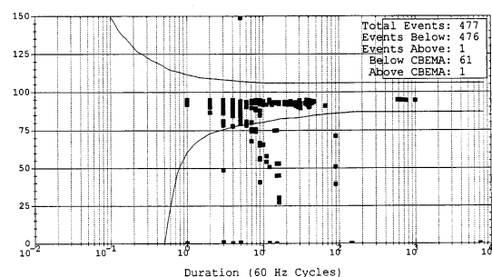
Fig. 2. Comparison of voltage sags with the CBEMA curve
