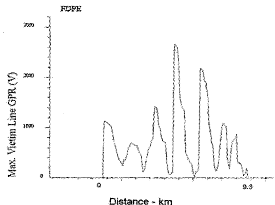
Figure 5: Coating Stress Voltage with insulating joints
