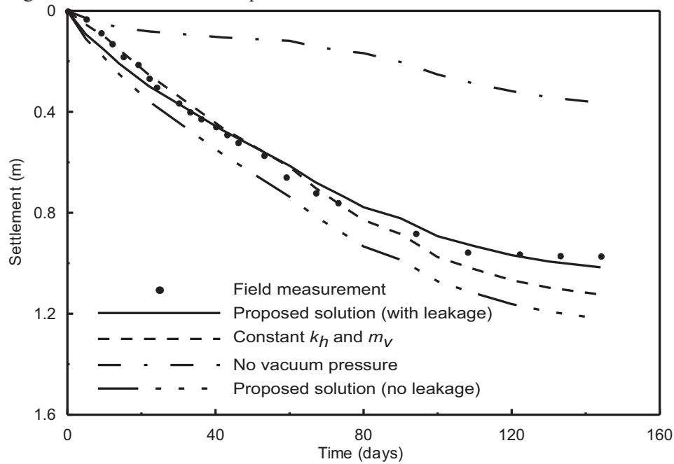
Figure 12 Surface settlement predictions at the centerline of Embankment TV2
