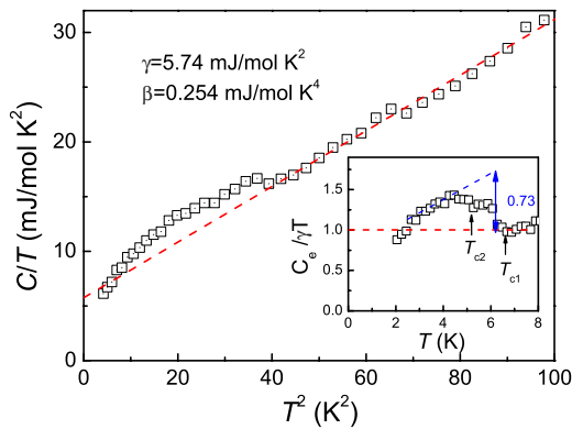
FIG. 4. (Color online) Curve of C/T versus T^2 for the sample of x=0.04 in LaFe 1-x Ni x AsO system under zero field. The inset shows C_e/\gamma T as a function of temperature, where C_e denotes electronic specific heat.
