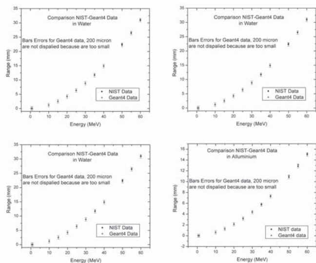
Fig. 3. Comparison between simulated and tabulated by NIST range of proton beams
