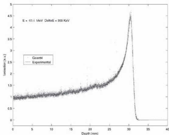
Fig. 4. Comparison between simulated and experimental Bragg curve in water of 62 AMeV proton beams
