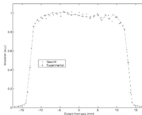
Fig. 5. Simulated and experimental lateral dose distribution for proton beams at the patient position
