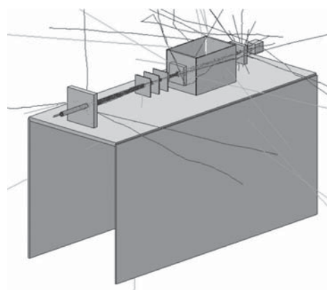
Fig. 2. The proton therapy beam line as it is simulated and displayed by hadronTherapy application
