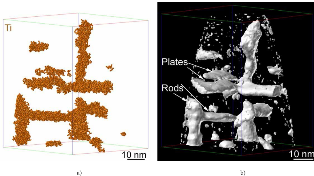
Fig. 4. Ti map (a) and 40% (Ni+Ti) iso-concentration surfaces (b) showing formation of predominantly (\text{Fe,Ni})_3\text{Ti} precipitates in martensite after 600 s ageing at 550^\circ\text{C} . All other atoms removed by maximum separation method in a).
