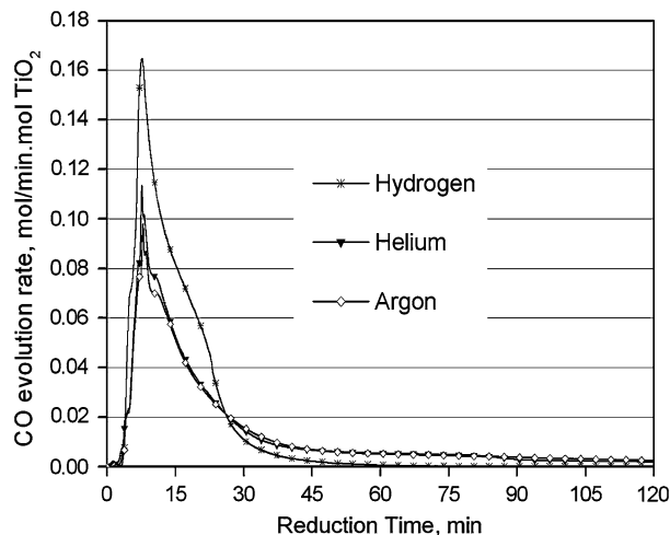
Fig. 14—Effect of gas atmosphere on CO evolution at 1400 °C.
