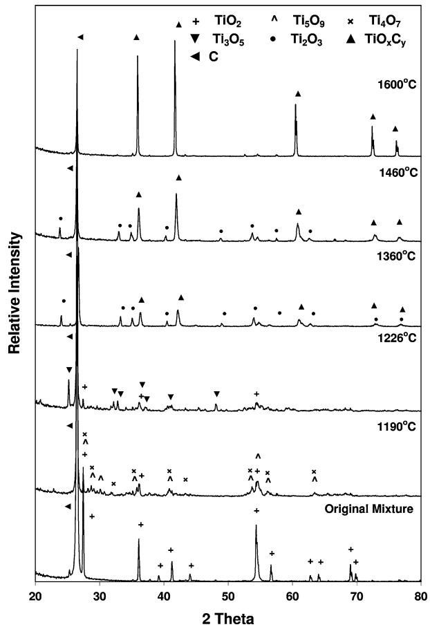
Fig. 3—XRD patterns of samples in the progress of temperature-programmed reduction in argon. The furnace temperature was ramped from 350 °C at 3 °C/min.
