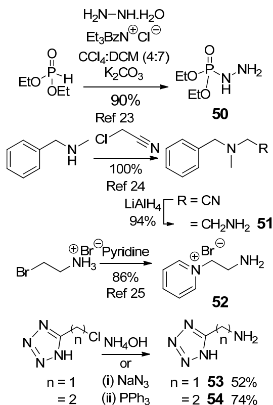
Scheme 3. Synthesis of non-commercially available amines 50-54 . 23-25
