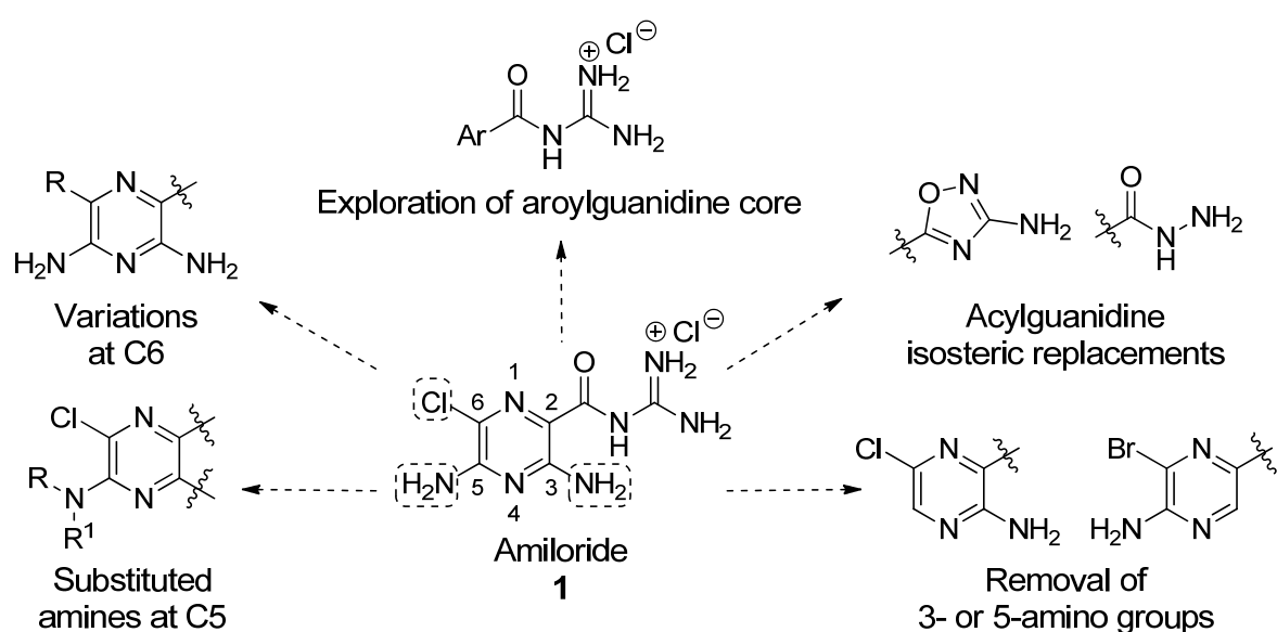
Figure 2. Summary of the amiloride structural features examined.
