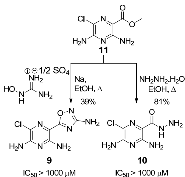
Scheme 1. Analogs incorporating acylguanidine isosteres.
