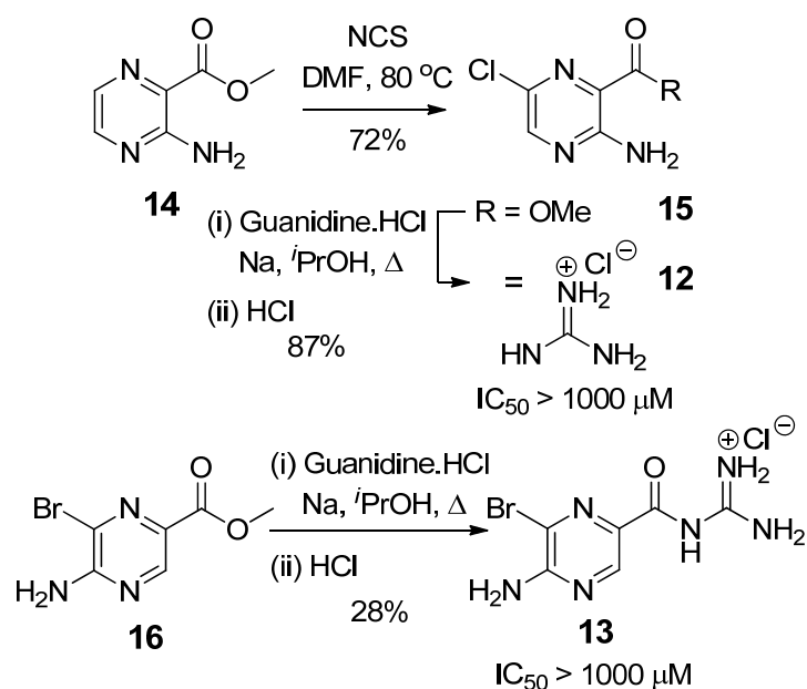
Scheme 2. Analogs with 3- and 5-amino groups removed.
