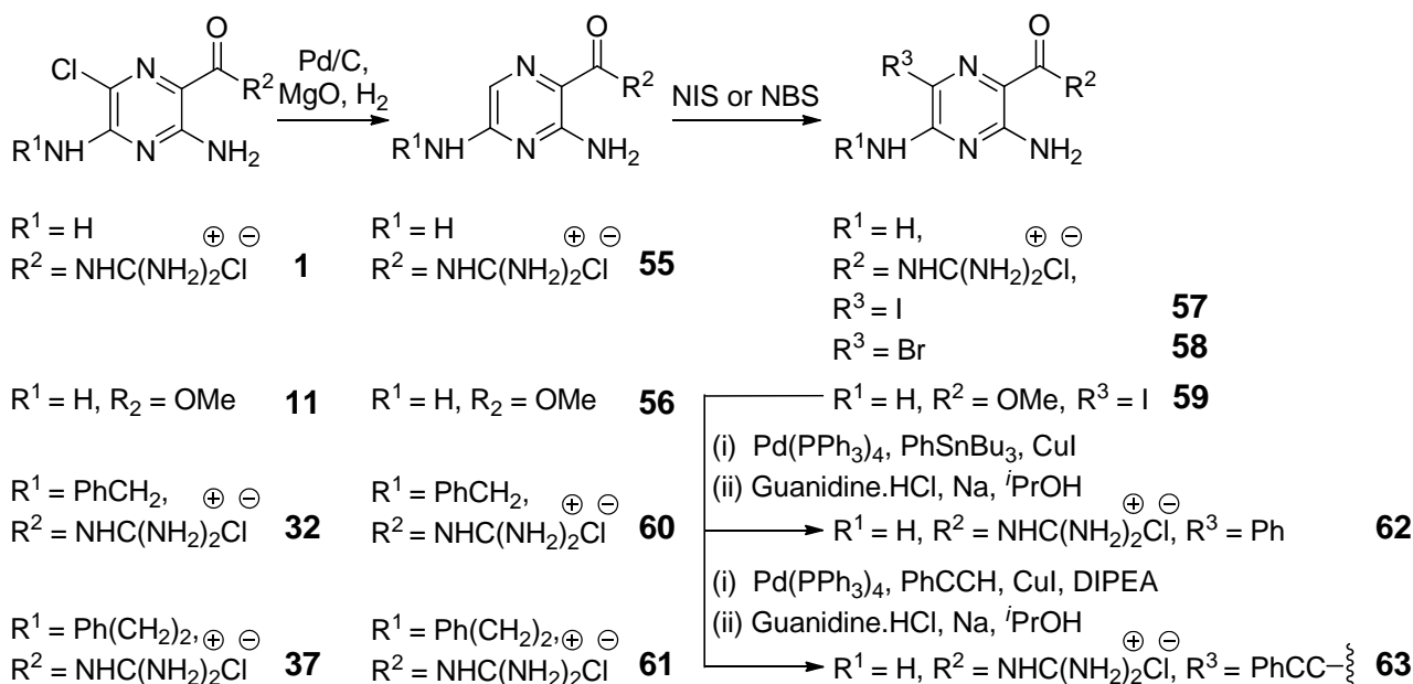
Scheme 4. Synthesis of analogs with variations at C6.
