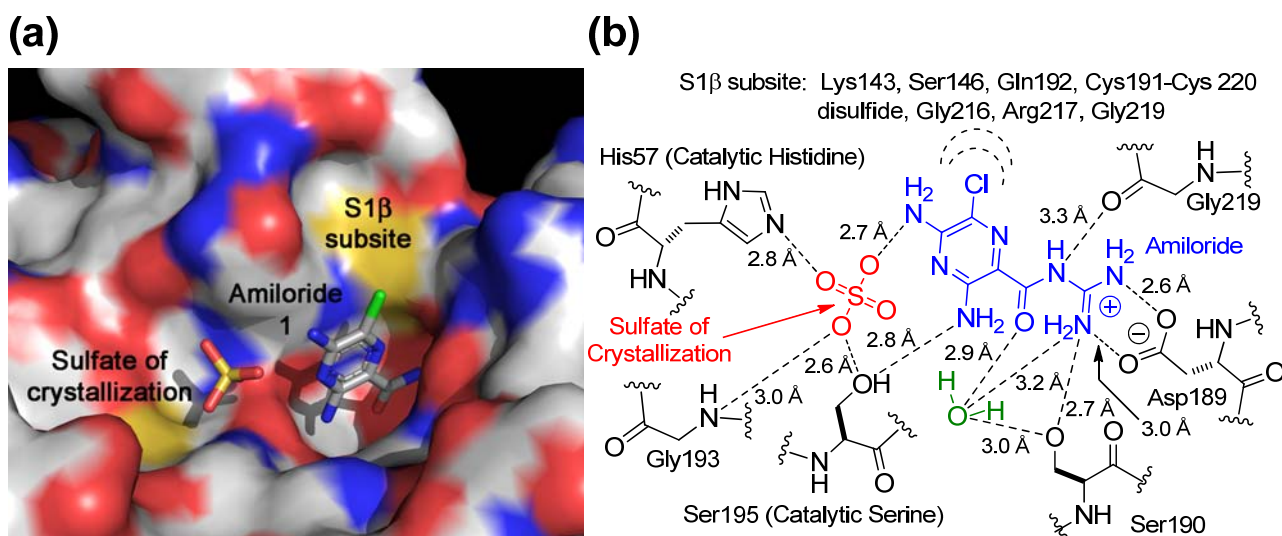
Figure 1. (a) X-ray crystal structure of the amiloride 1 :uPA complex (binding site only); PDB 1f51. 16 (b) Summary of the binding interactions between amiloride (blue), uPA (black), an adventitious sulfate of crystallization (red) bound in the oxyanion hole and a water molecule (green) bound deep within the S1 pocket.
