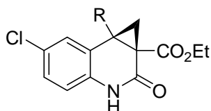
9 ; R = alkyl
