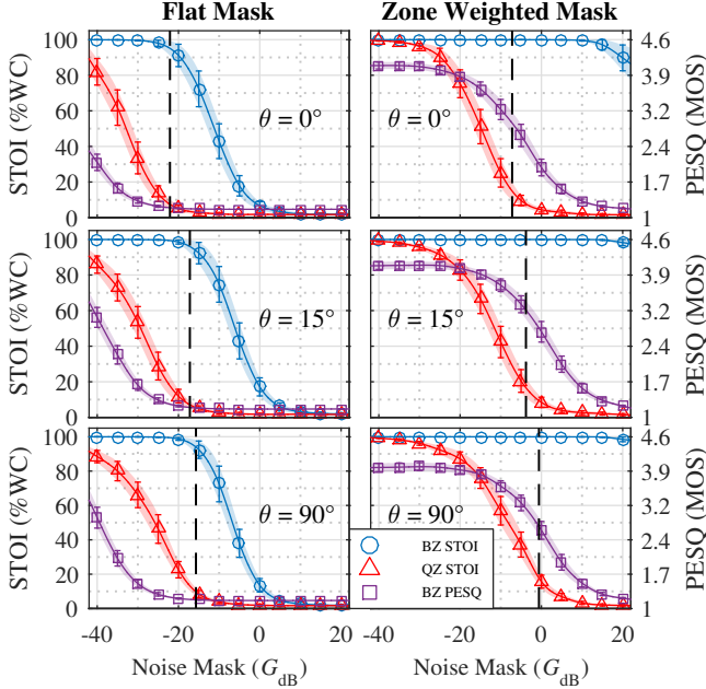
Fig. 2. Mean STOI and PESQ are shown for the anechoic environment and 95% confidence intervals are indicated. BZ and QZ are the bright and quiet zone, respectively. Black dashed lines indicate optimum G_{dB} and \lambda = 1 .
