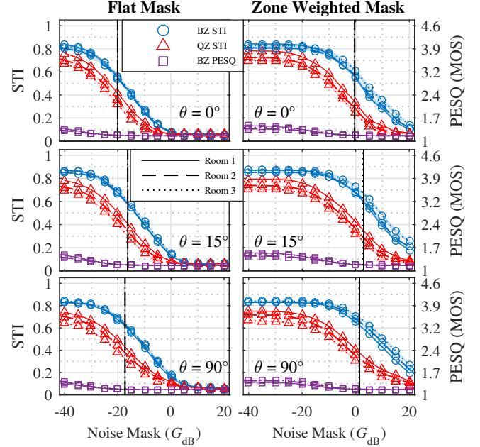
Fig. 3. Mean STI and PESQ are shown for the small office, medium office and restaurant/café labelled as Room 1, Room 2 and Room 3, respectively. BZ and QZ are the bright and quiet zones, respectively. Vertical black lines indicate optimum G_{dB} and \lambda = 1 .
