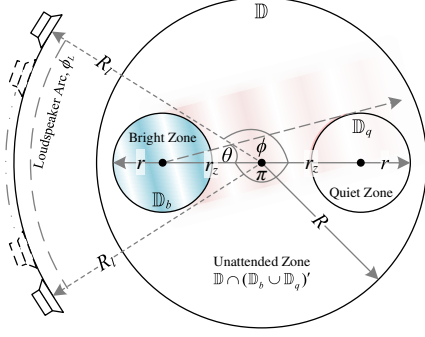
Fig. 1. A weighted multizone soundfield reproduction layout is shown. The shading depicts the desired bright zone soundfield partially directed towards the quiet zone causing the occlusion problem.
