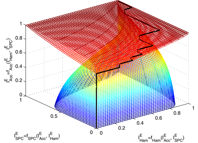
Figure 3. Three-dimensional EXIT chart for Hamming(31,26)-SPC(32,31)-Accumulate code at E_b/N_0 = 3.19 dB
