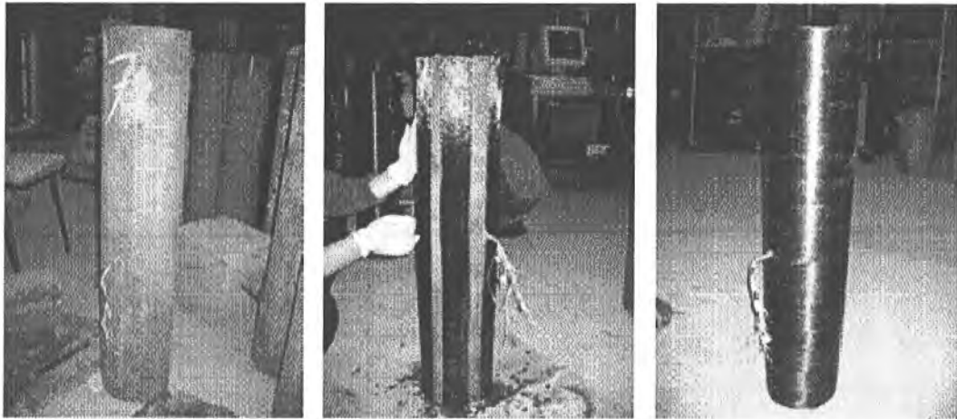
Fig. 3 External confinement application.
