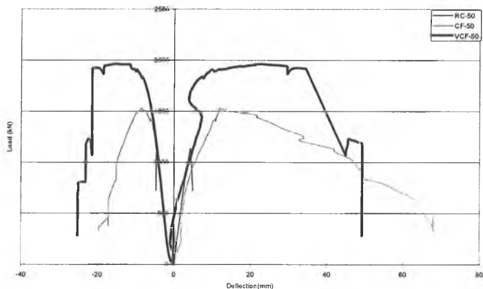
Fig. 8 Load-deflection for Specimens RC-50, CF-50 and VCF-50.
