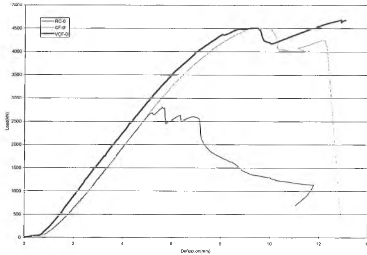
Fig. 6 Load-deflection for Specimens RC-0, CF-0 and VCF-0.
