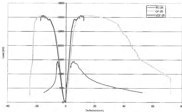
Fig. 7 Load-deflection for Specimens RC-25, CF-25 and VCF-25.
