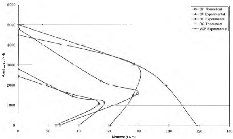
Fig. 13 Interaction diagrams for the tested specimens.
