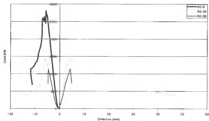
Fig. 9 Load-deflection for Specimens RC-0, RC-25 and RC-50.
