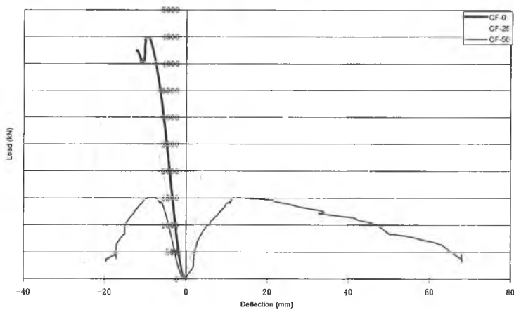
Fig. 10 Load-deflection for Specimens CF-0, CF-25 and CF-50.
