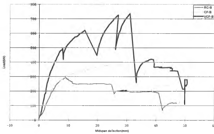
Fig. 12 Load-deflection for Specimens RC-B, CF-B and VCF-B.
