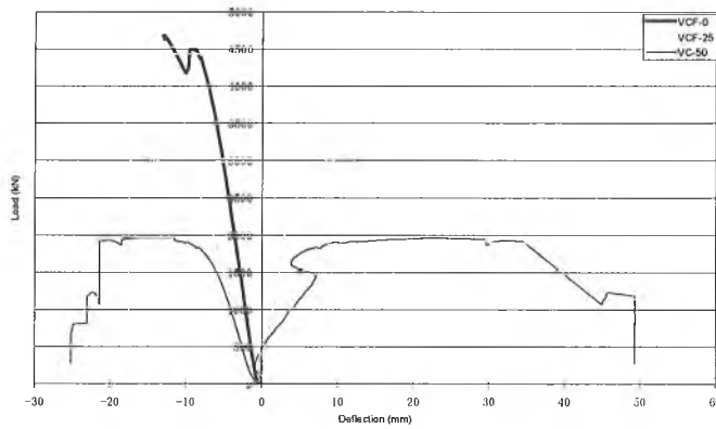
Fig. 11 Load-deflection for Specimens VCF-0, VCF-25 and VCF-50.
