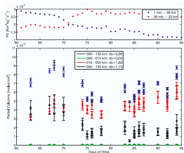
Figure 5. NO partial columns retrieved over Eureka. PV indicates disturbed dynamic conditions near day 70.
