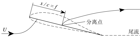
图2 Kirchhoff 流中平板分离流的后缘分离点位置 Fig.2 The trailing edge separation point f defined in the Kirchhoff flow past a fiat plate
