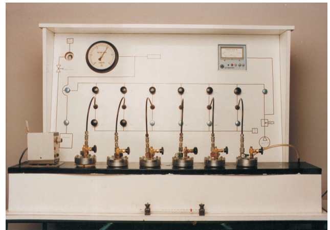
FIG 1 - High pressure sorption/desorption apparatus.
