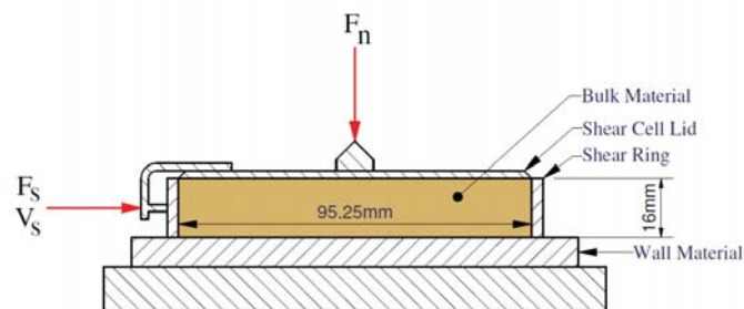
Fig. 1 Schematic of the standard Jenike wall friction test arrangement
