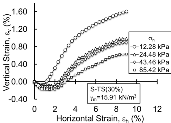
Fig.5 Variation of vertical strain with horizontal strain for different normal stress
