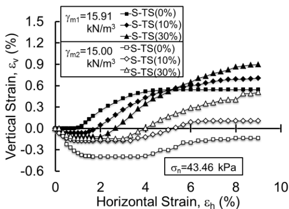
Fig.8 Variation of vertical strain with horizontal strain for different sand matrix unit weight
