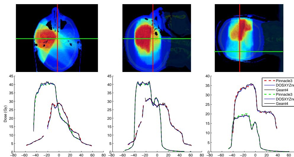
Figure 3. IMRT plan comparison for a 4 field (54 segment) brain IMRT plan.
