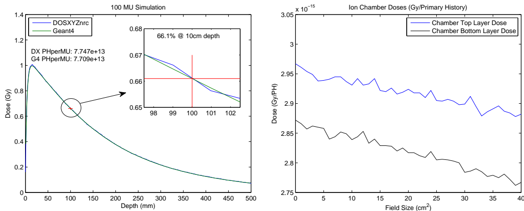
Figure 2. Left: Absolute calibration simulation results. An excellent match is seen between Geant4 and DOSXYZnrc. Right: Monitor chamber doses for symmetric beams from 0x0 cm 2 to 40x40 cm 2 .
