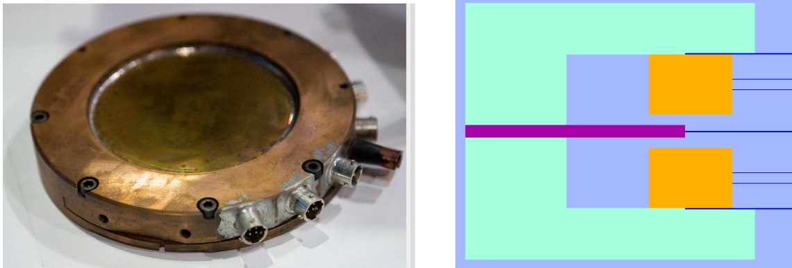
Figure 1. Left: Image of the Varian monitor chamber. Right: Implementation of the monitor chamber in BEAMnrc using two CHAMBER component modules.
