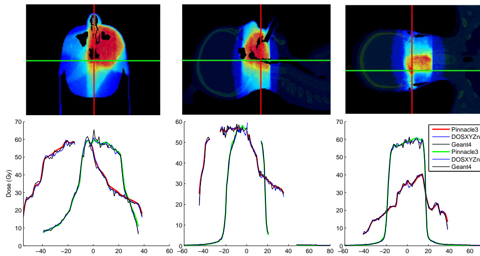
Figure 4. IMRT plan comparison for a 4 field (54 segment) nasopharynx IMRT plan.
