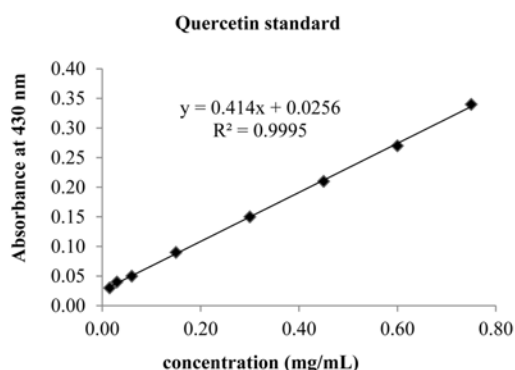
Figure 4. Calibration plot for flavonoid determination.
