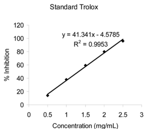
Figure 2. Calibration plot for ABTS assay.
