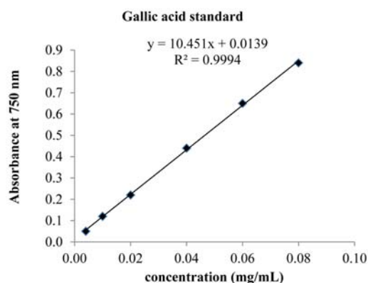
Figure 3. Calibration plot for phenolic determination.
