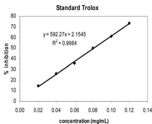
Figure 1. Calibration plot for DPPH assay.
