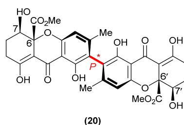
Figure 7: The determined absolute stereochemistry of naturally produced rugulotrosin A ( 20 ).
