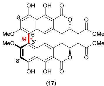
Figure 6: The confirmed structure of the naturally produced ( M )-viriditoxin (17).
