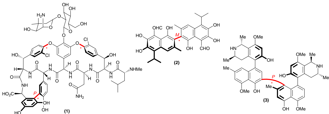
Figure 1: The structure of vancomycin B (1), the active ( M )-gossypol (2), and Mbandakamine A (3), with chiral axes shown in red.
