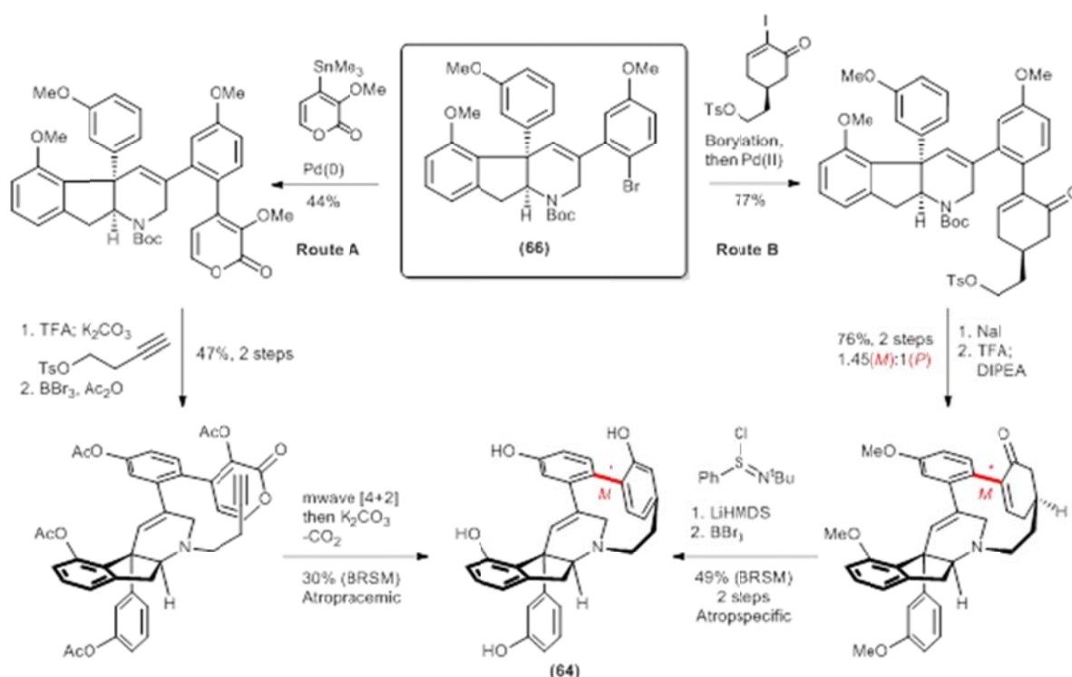
Scheme 12: The first- ( Route A ) and second-generation ( Route B ) syntheses of Haouamine A by the Baran group.
