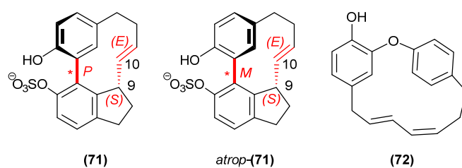
Figure 15: The structure of Tedarene B ( 71 ) in the native ( P ) configuration, and its ( M ) atropenantiomer ( atrop-71 ), hindered by both its 10-( E ) and 9-( S ) stereochemistry. Tedarene A ( 72 ) was also isolated, though found to be an atropisomeric due to an insufficient rotational energy barrier about the diene.
