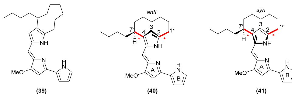
Figure 11: The initial incorrect structure (butylcycloheptylprodiginosin, BCHP) attributed to streptorubin B ( 39 ), and the confirmed absolute structures of major natural product (7' S , anti ) streptorubin B ( 40 ) and the minor product (7' S , syn ) streptorubin B ( 41 ), with the minor (7' R , anti ) isomer not shown.
