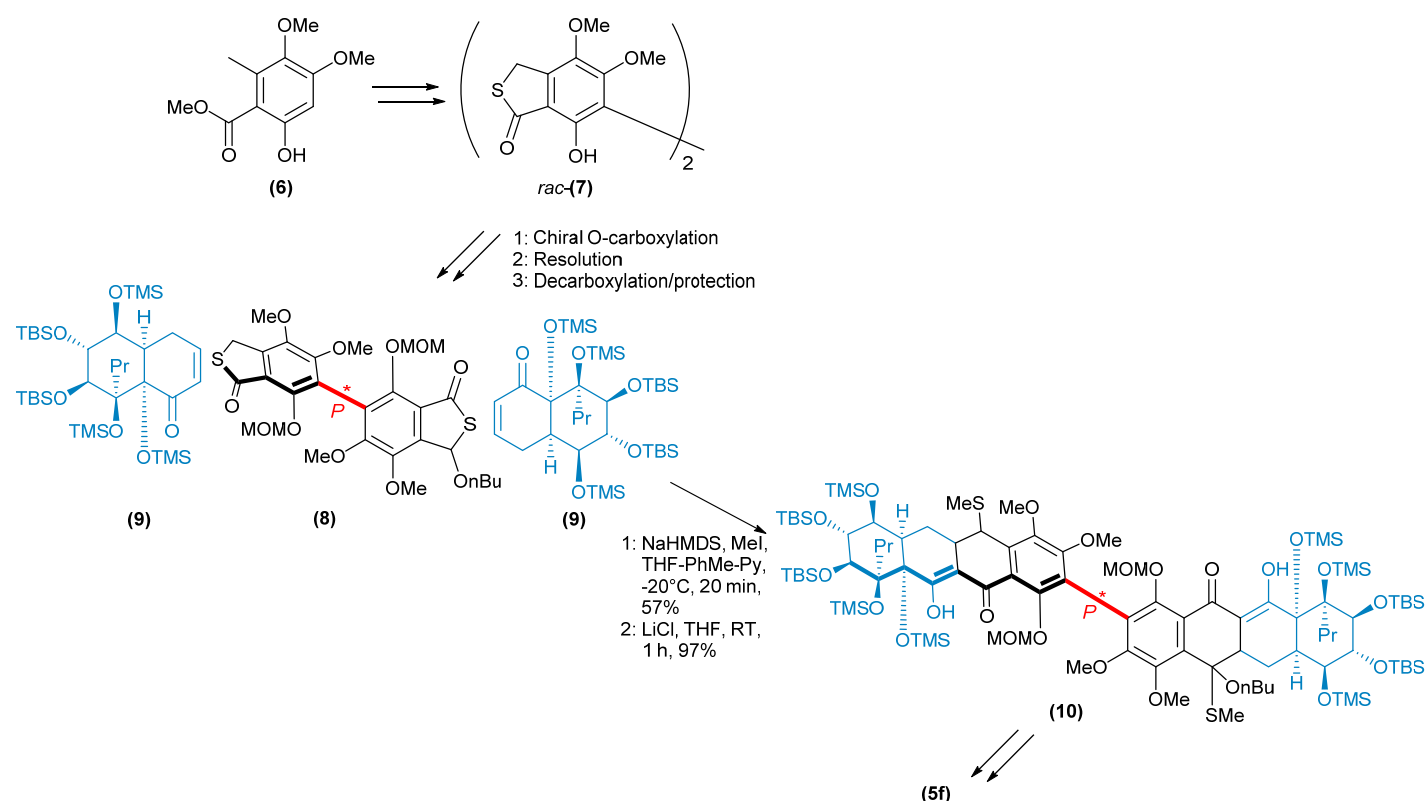
Scheme 1: The first synthesis of hibarimicinone ( 5f ), with construction of the hibarimicin core by a dual-Michael-Dieckmann reaction of central thiolactone 8 with 9 , furnishing the final product 5f after deprotection.
