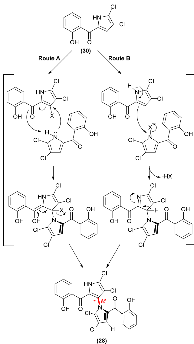
Scheme 6: Proposed mechanisms for the enzymatic synthesis of marinopyrrole A, utilising either ( Route A ) C-halogenation and nucleophilic substitution, or ( Route B ) N-halogenation and electrophilic substitution. For both cases, X = a halogen (Cl, Br, I)
