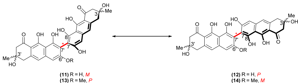
Figure 4: The determined structures of flavomannin A ( 11 ), flavomannin B ( 12 ), flavomannin C ( 13 ), and flavomannin D ( 14 ), with undetermined point chirality at C3 and C3'. 11 and 12 are homodimers comprised of two atrochryson moieties connected via the atropisomeric bond; whereas 13 and 14 are heterodimers comprised of an atrochryson moiety (right of atropisomeric bond) and an ether derivative of atrochryson (left of atropisomeric bond).
