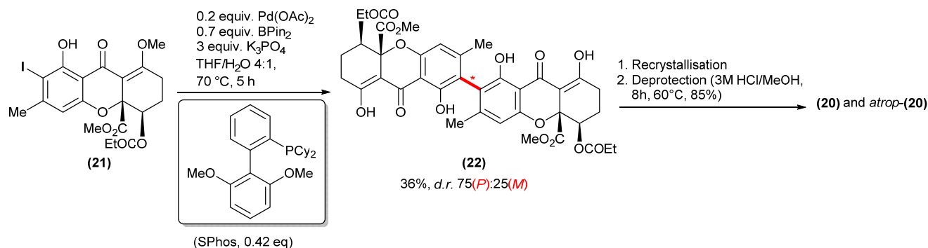
Scheme 3: Atropselective synthesis of rugulotrosin A ( 20 ) and atrop -rugulotrosin A by Qin et al. This approach utilises point-to-axial transfer using an achiral ligand during a one-pot Suzuki coupling of monomer 21 to generate protected dimer 22 in 36%, with a d.r. of 75( P ):25( M ). These intermediates were separated using recrystallization, and following deprotection afforded rugulotrosin A and atrop -rugulotrosin A in 85% each.
