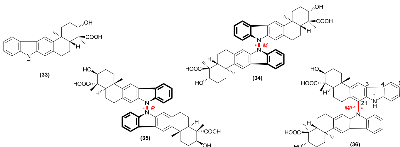
Figure 10: The known structure of xiamycin A ( 33 ), and determined structures of dixiamycin A ( 34 ), dixiamycin B ( 35 ), and an unnamed C-N linked xiamycin dimer ( 36 ), of which both the M and P isomers were isolated.
