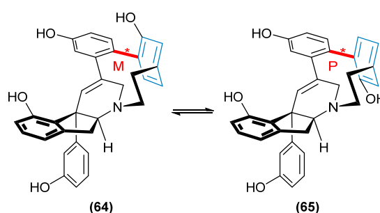
Figure 13: The structure of Haouamine A (64) and its atropisomer (65), with the highly uncommon distorted benzene ring shown in blue.
