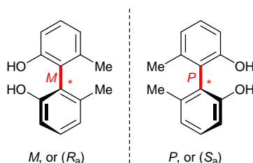
Figure 1: Restricted rotation about a biaryl bond, giving rise to ( M ) and ( P ) atropisomers, with alternate nomenclature of R_a and S_a respectively (subscript a indicating axial chirality), with highest priorities assigned to the ortho hydroxyl groups.
