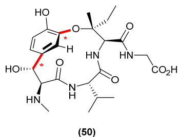
Figure 12: The absolute structure of ustiloxin D (50), as determined by NOE spectroscopy, with likely key bonds regarding atropisomeric nature indicated with an asterisk (*).
