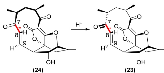
Figure 8: The absolute configuration of abyssomicin C ( 23 ) and atrop-abyssomicin C ( 24 ), which may convert to 23 under mild acidic conditions.
