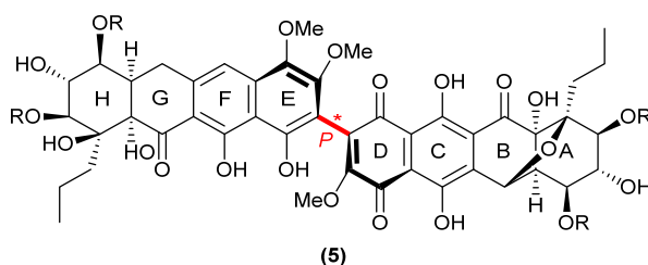
Figure 3: The general structure of the hibarimicin family of molecules; hibarimicins (A, B, C, D, G) R = Sugar (5a-e); hibarimicinone R = H (5f).
