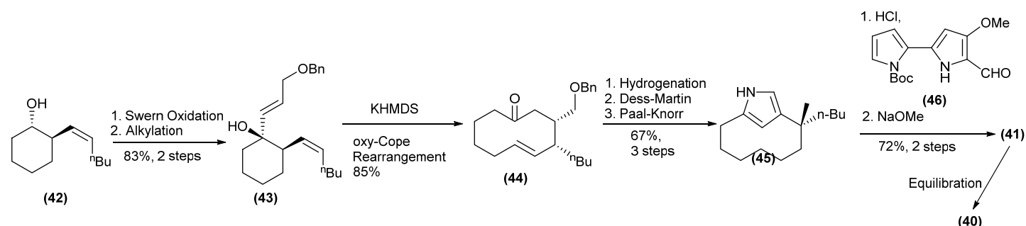
Scheme 8: The first total-synthesis of streptorubin B, the main product being the syn isomer ( 41 ), which equilibrated over time to give the more stable anti configuration ( 40 ).
