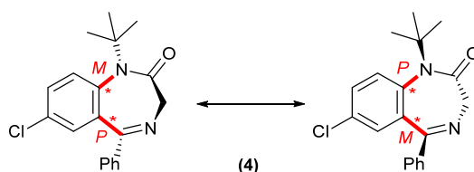
Figure 2: The two possible configurations of benzodiazepine (4).
