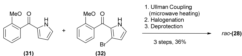
Scheme 5: Convergent total synthesis of racemic marinopyrrole A ( 28 ).
