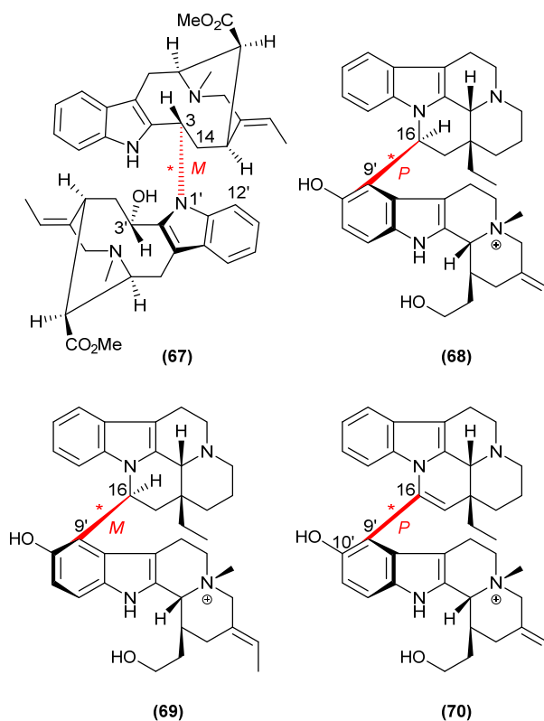
Figure 14: Determined structures of bisnicalaterines A ( 67 ), B ( 68 ), C ( 69 ), and D ( 70 ), and the stereochemistry about each axis.
