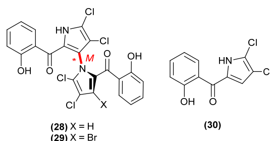
Figure 9: The absolute structures of marinopyrroles A ( 28 ) and B ( 29 ), with their composite monomeric precursor monodeoxyoluteolin ( 30 ).
