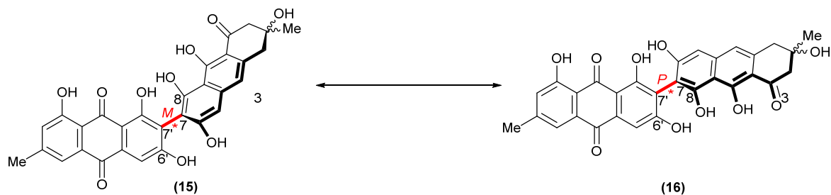
Figure 5: The determined structures of talaromannin A ( 15 ), and talaromannin B ( 16 ), with unknown point chirality of C3. The heterodimer is comprised of an emodin moiety (left of atropisomeric bond) and atrochryson moiety (right of atropisomeric bond).
