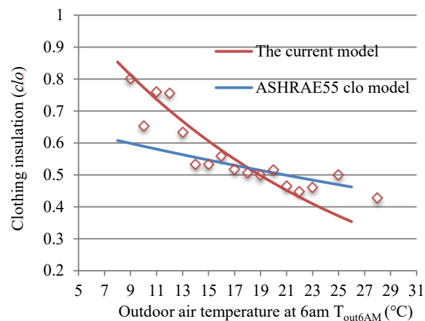
Figure 2. Clothing behaviour observed in the current study compared against the ASHRAE55 dynamic clothing insulation model as a function of outdoor temperature at 6AM
