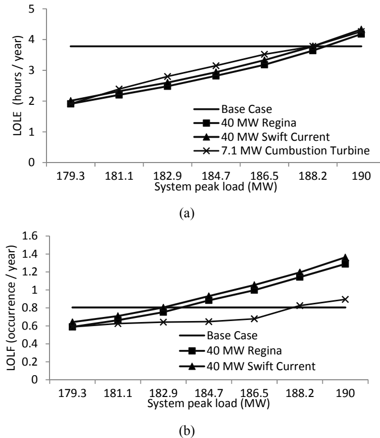
Fig. 4. ELCC obtained using LOLE and LOLF: (a) LOLE index; (b) LOLE index.
