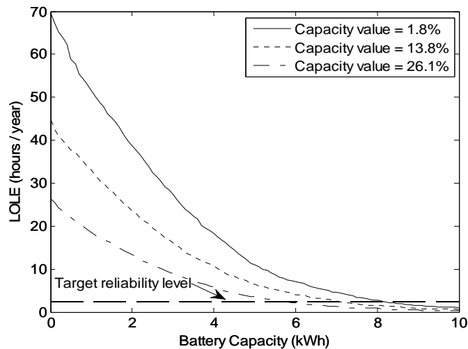
Fig. 3. Impact of storage on RAPS system reliability
