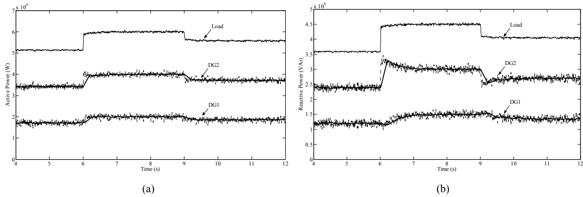
Fig.6. RAPS system with two inverter-based generators: a. Active power sharing. b. Reactive power sharing
