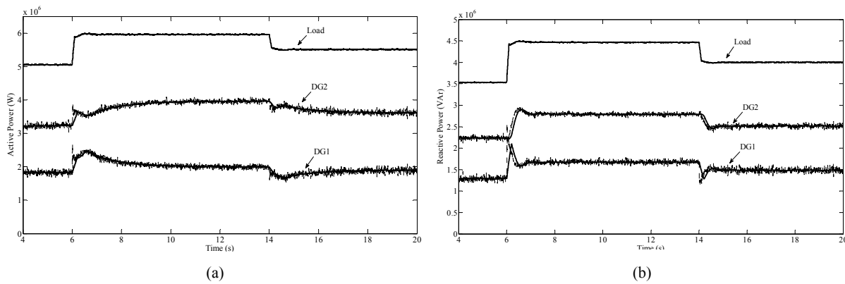
Fig.7. RAPS system with conventional and inverter-based generators: a. Active power sharing. b. Reactive power sharing
