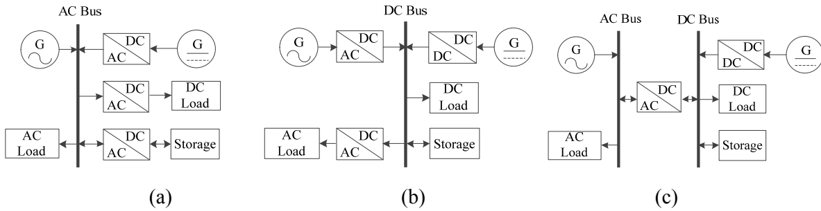
Fig. 2. RAPS system topologies: (a) Common AC-bus scheme; (b) Common DC-bus scheme; (c) Hybrid-bus scheme.
