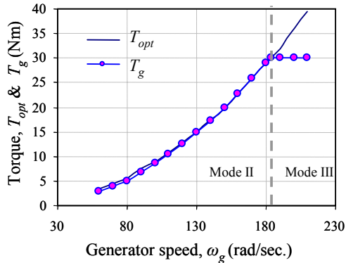
Figure 7. Optimum torque and generator torque.
