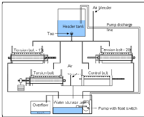
Figure 1 – The general layout of the bolt corrosion rig
