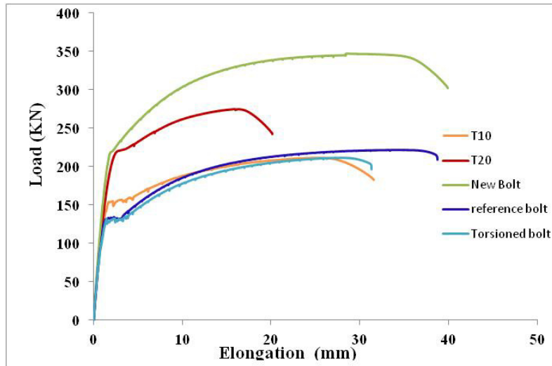
Figure 6 – Load displacement profiles of various bolts
