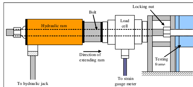
Figure 3 – Axial tensioning of bolts installed in the tension rig of Figure 2
