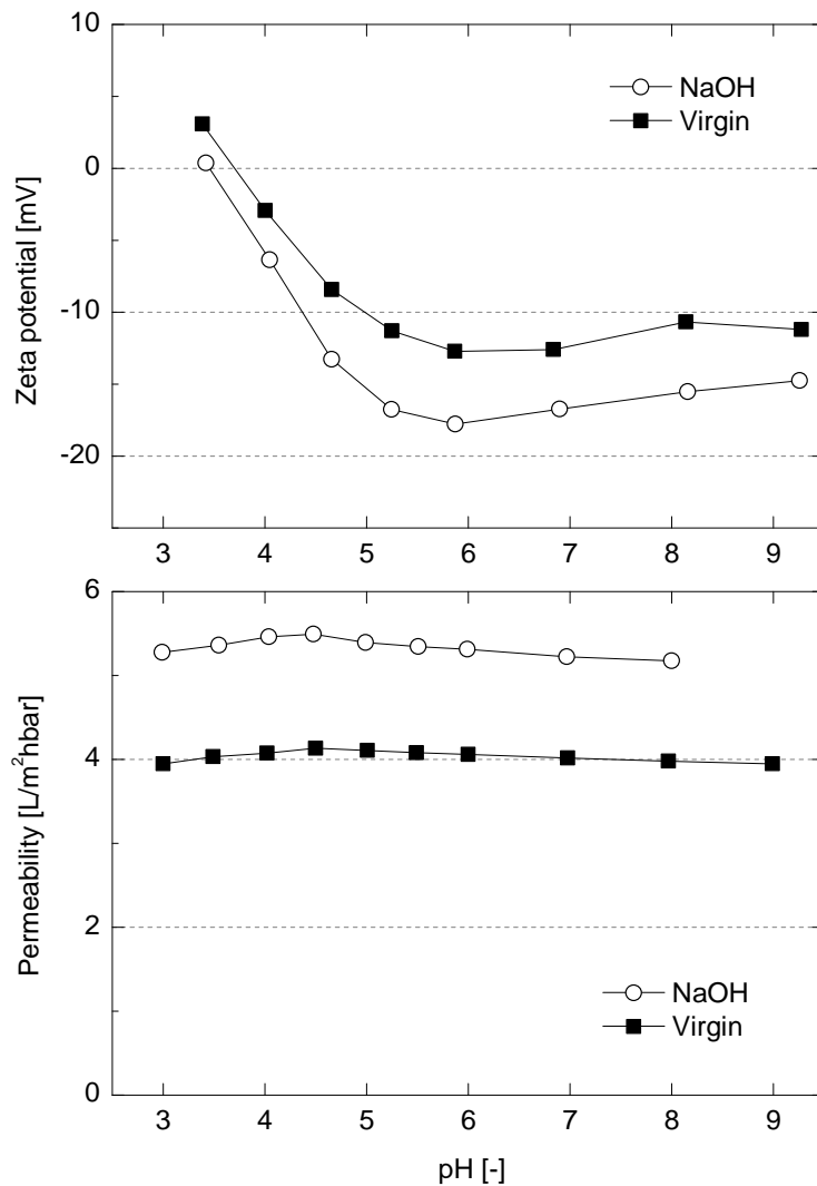
Figure S6: (a) Zeta potential and (b) permeability of TFC-HR membrane before and after being exposed to NaOH (pH 12) solution for 25 hours at 30 °C. The analysis of zeta potential was carried out in 1mM KCl solution. Pure water permeability was determined with Milli-Q water at 1,000 kPa and 20°C feed temperature.
