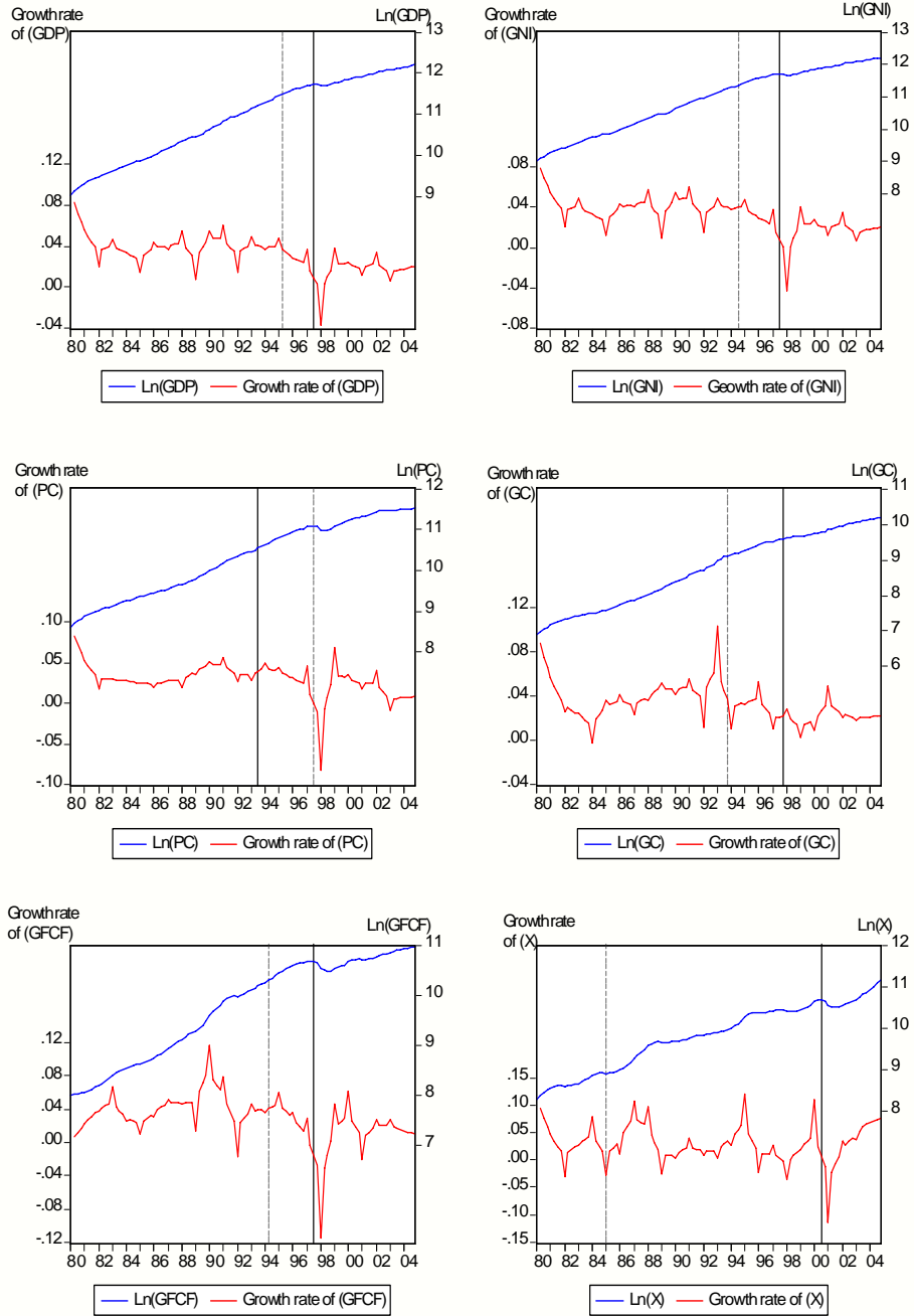
Figure 1 Plots of the Series and Estimated Timing of Structural Breaks
