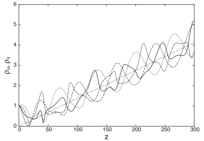
FIG. 2. Radial positions of nematicons for the initial values a_u=1.8 , a_v=1.8 , w_u=3.0 , w_v=3.0 , \xi_u=1.0 , \xi_v=-1.0 , \eta_u=\eta_v=0.0 , U_u=0.03 , U_v=-0.01 , V_u=0.03 , V_v=-0.01 with \nu=500 , q=2 , A_u=1.0 , A_v=0.95 , D_u=1.0 , D_v=0.98 . Full numerical solution, u color (—); v color (---); solution of modulation equations for u color ( \cdot\cdot\cdot ); v color (— · — · —); momentum conservation result (35) (— · — · —).
