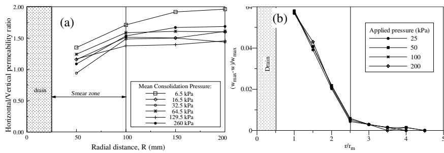
Figure 6. Smear zone determination (a) permeability approach (Indraratna and Redana, 1998) (b) water content approach (Sathananthan and Indraratna, 2006) ( w = water content)
