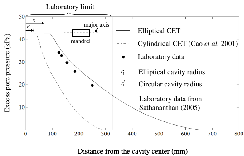
Figure 7. The patterns of distribution s predicted for excess pore pressure with the radial distance using elliptical CET and cylindrical CET along the major axis of the mandrel 0.5m below the soil surface, and measured when the tip of the mandrel's shoe passed the horizontal plane under consideration, with a preconsolidation pressure = 30 kPa (Ghandeharioon et al. 2010)
