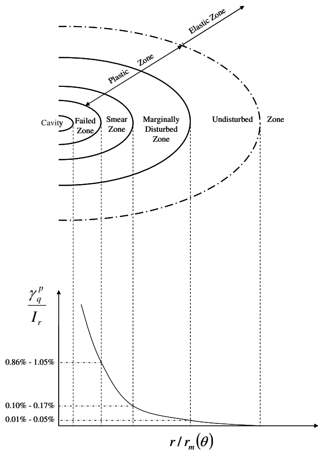
Figure 8. The distribution pattern for the ratio of the plastic shear strain to the rigidity index in relation to the radial distance normalised by the equivalent elliptical radius of the mandrel characterising the disturbed soil surrounding a PVD (Ghandeharioon et al. 2010)
