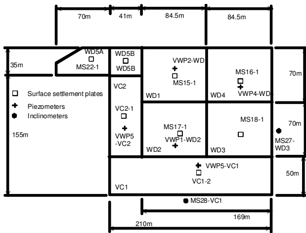
Figure 13. Site layout for S3A with instrumentation plan (Indraratna et al. 2011)
