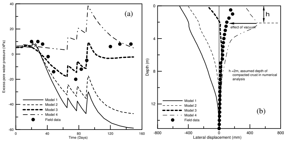
Figure 12. (a) Excess pore pressure predictions and (b) lateral displacement predictions (Indraratna et al. 2004)
