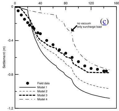
Figure 11. (a) Stage loading (b) variation of vacuum with time for Model 3 and (c) settlement predictions (Indraratna et al. 2004)
