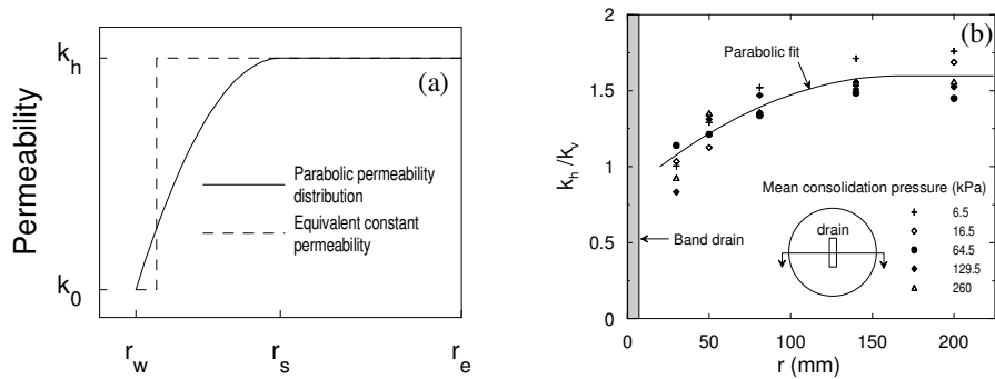
Figure 3. (a) Permeability distribution and (b) ratio of horizontal to vertical permeability ( k_h/k_v ) along radial distance from drain in large scale consolidometer (Walker and Indraratna, 2006) ( r_e=d_e/2 , r_s=d_s/2 and r_w = d_w/2 )
