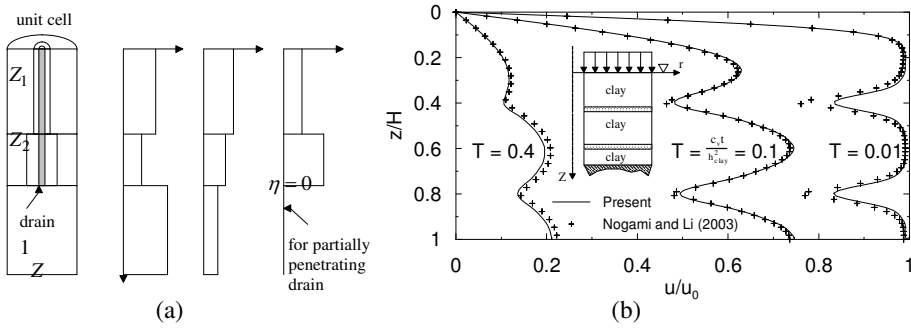
Figure 5. (a) Multi-layered consolidation properties and (b) model verification: multi-layer equal-strain vs free-strain (Walker et al. 2009)
