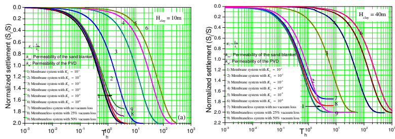
Figure 9. Normalised settlement-time factor curves for varying the permeability of the sand blanket (for membrane system) and the loss of vacuum (for membraneless system): (a) the thickness of the clay is 10 m; (b) the thickness of the clay is 40 m (after Geng et al. 2012)
