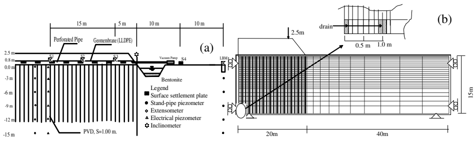
Figure 10. (a) Cross-section of an embankment with profile of the subsoil and (b) finite element discretisation of the foundation of the embankment (Indraratna et al., 2004)
