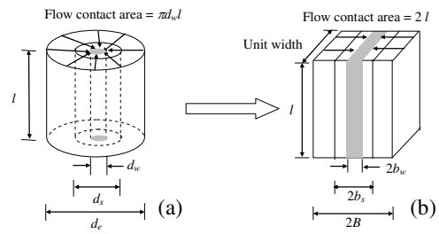
Figure 4. Unit cell analysis: (a) axisymmetric condition, (b) equivalent plane strain condition (after Indraratna et al., 2005a) ( B , b_s , b_w = half width of unit cell, smear zone and drain, respectively under plane strain condition)
