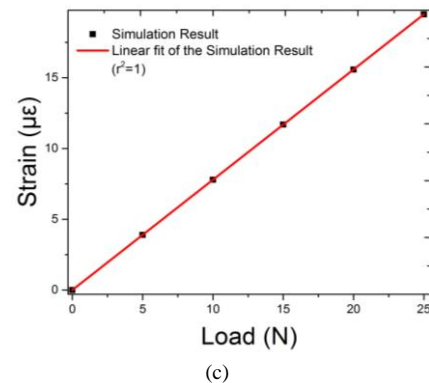
Fig. 5. (a) Strain profile of the packaged sensor with applied load (b) strain experienced by the embedded optical fibre (c) simulated load vs. strain plot of the packaged sensor
