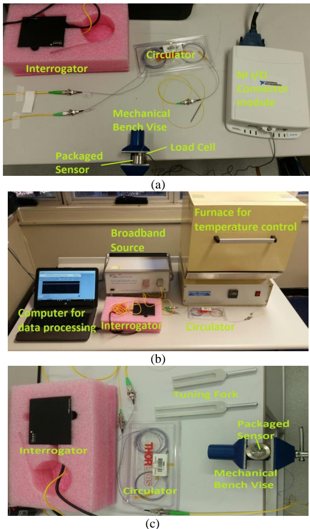
Fig. 6. The photographs of the set up for characterisation (a) load (b) temperature (c) vibration
