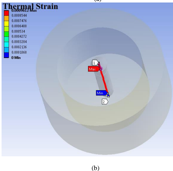
Fig 4. (a) Thermal strain profile of the packaged sensor due to applied temperature (b) the thermal strain along the embedded fibre containing the FBG
