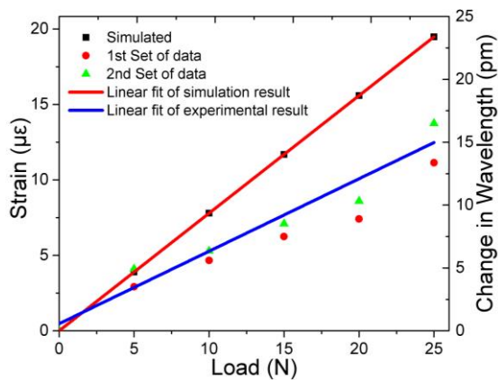
Fig. 7: Measured wavelength shift and calculated strain due to applied load calculated strain from the experiment due to applied load and its comparison with the simulation
