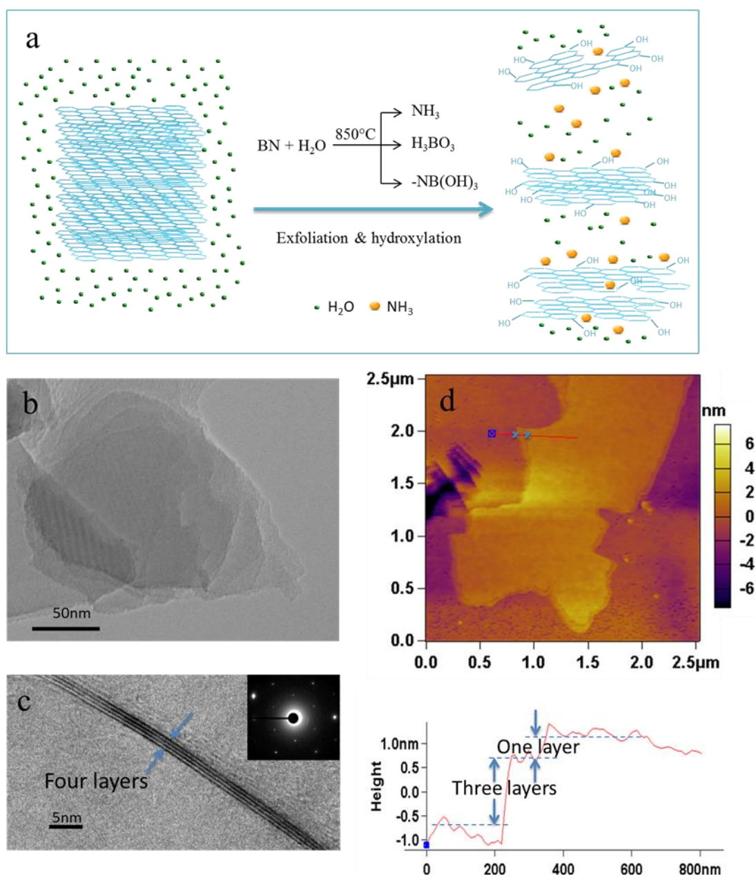
Figure 1. a) Schematic illustration of hydrolysis-assisted exfoliation and hydroxylation of h -BN powder in hot steam, where \text{H}_2\text{O} reacts with h -BN, forming \text{NH}_3 and \text{-NB(OH)}_x , and the highly energetic \text{H}_2\text{O} and \text{NH}_3 assist the exfoliation through diffusion between BN layers; b) TEM image of a Moiré pattern due to the stacking of few-layered OH-BNNS; c) TEM image of four-layered OH-BNNS (inset showing the corresponding electron diffraction pattern); d)
