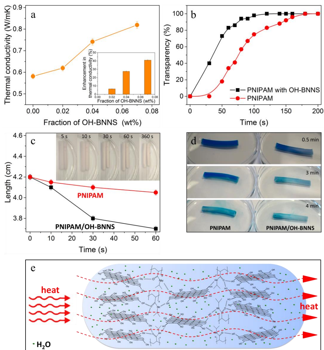
Figure 5. a) Thermal conductivity improvement with the ratio of OH-BNNS (inset: the improvement by percentage), b) change in transparency, c) change in length of cylindrical samples (inset: photographs of hydrogels at different times, with PNIPAM on the left and PNIPAM/OH-BNNS on the right), d) dye release upon heating, and e) schematic illustration of the enhanced heat transfer in PNIPAM/OH-BNNS hydrogel, which has resulted from the excellent integration between the OH-BNNS, H 2 O, and the cross-linked PNIPAM through hydrogen bonding.
