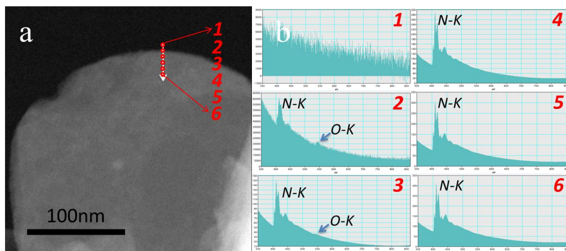
Figure 3. EELS mapping shows that the hydroxyl groups are predominately located along the edges of the nanosheets. Area 1 is off the BNNS so no O-K or N-K peaks are observed; on moving to the edge of the BNNS (area 2), the O-K peak appears and then becomes weaker on moving away from the edge (area 3). The O-K peak is not observed when moving further into the basal plane (areas 4, 5, and 6). The presence of 1s- \pi^* and 1s- \sigma^* peaks of the N-K edge confirm that the intrinsic hexagonal structure of h -BN still remains.
