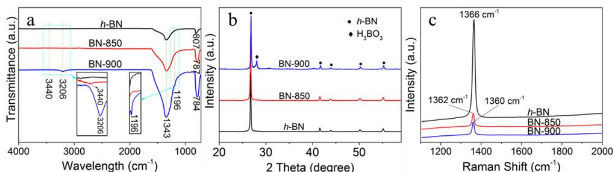
Figure 2. Pristine h -BN and h -BN treated at 850 °C (denoted as BN-850) and 900 °C (BN-900). a) FTIR spectra showing the presence of only -NB(OH) x in BN-850, as opposed to the large amount of H 3 BO 3 in BN-900; b) XRD patterns revealing the presence of H 3 BO 3 in BN-900, which is negligible in BN-850. c) The red-shifts in the Raman spectra of the E 2g peak indicate the formation of few-layered BN at elevated temperatures.
