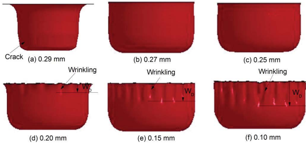
FIGURE 2. Simulation Results with Different Initial Blank Thicknesses
