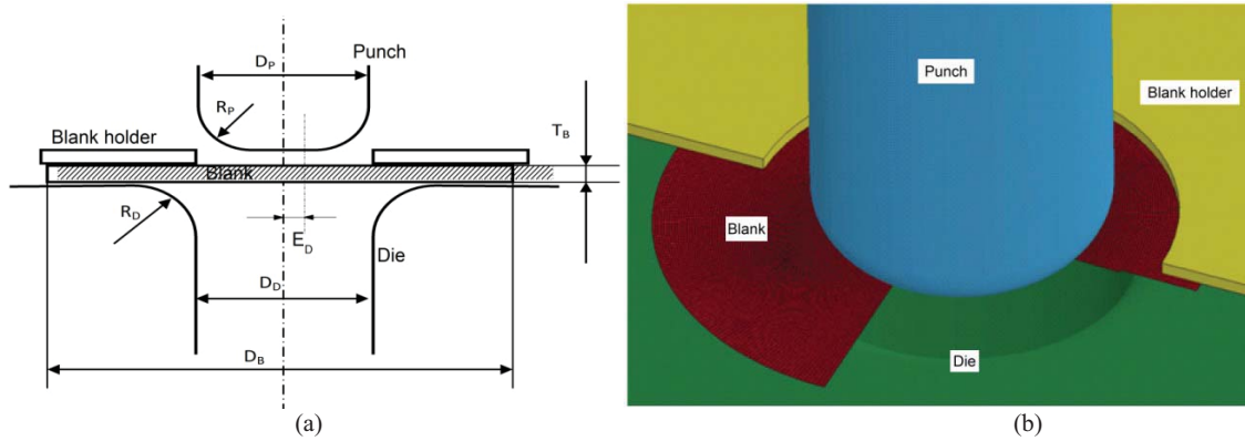
FIGURE 1. Geometric Dimensions and FE Model
