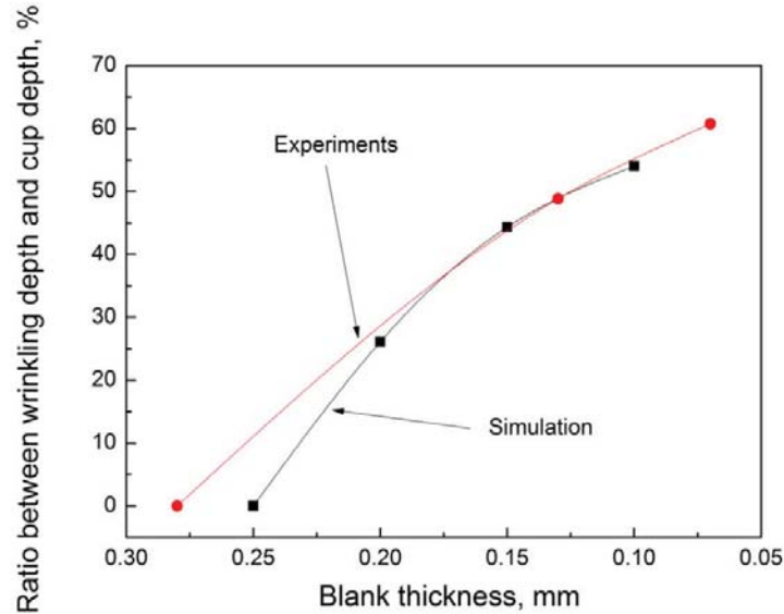
FIGURE 4. Wrinkling Depth under a Variety of Blank Thicknesses
