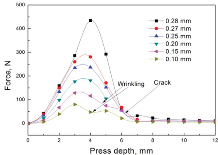
FIGURE 5. Punch Force during Deep Drawing under Different Blank Thicknesses
