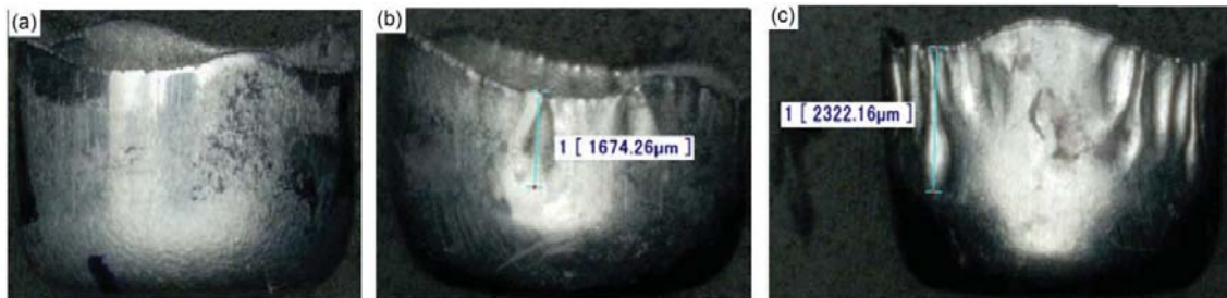
FIGURE 3. Experimental Samples with Blank Thickness (a) 0.28, (b)0.13, and (c) 0.07 mm
