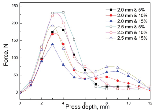
FIGURE 8. Punch Force during Deep Drawing under Different Eccentric Distances
