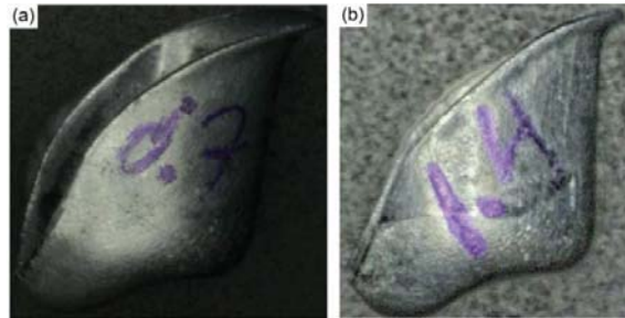
FIGURE 7. Experimental Samples with Eccentric 10% and 20% for Blank Thickness 0.28 mm
